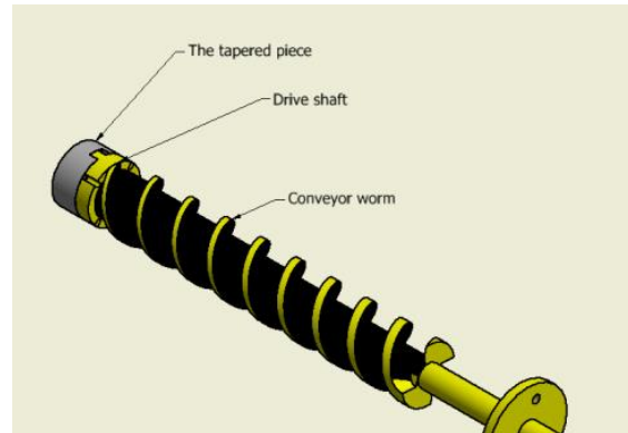
Fig. 7: Assembly consist in worm, washer and tapered piece
