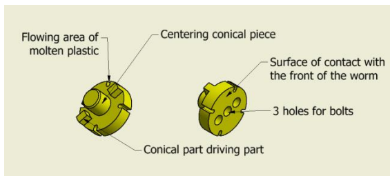
Fig. 5: Drive washer
