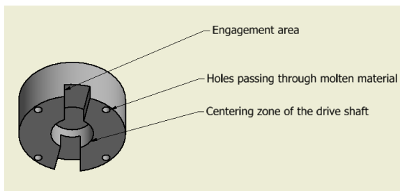
Fig. 6: The tapered piece
