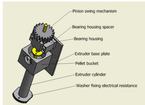
Fig. 8: Extruder without swinging mechanism
