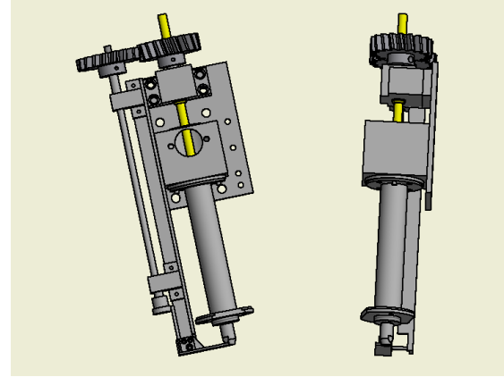
Fig. 3: Designed extruder
