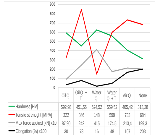
Fig. 6: Hardness and mechanical properties of high alloyed steel D2
