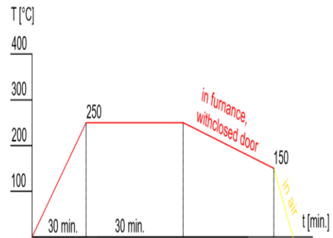
Fig. 4: Heat treating process for D2 (tempering)
