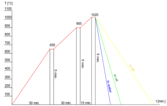
Fig. 3: Heat treating process for D2 (hardening)
