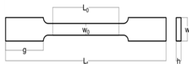
Fig. 1: Test specimen
