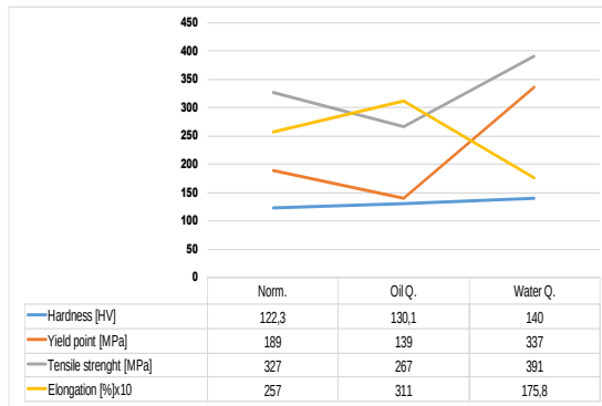
Fig. 5: Hardness and mechanical properties of low carbon steel C2D1 Measurements for D2 steel are presented below (Table 5, 6).
