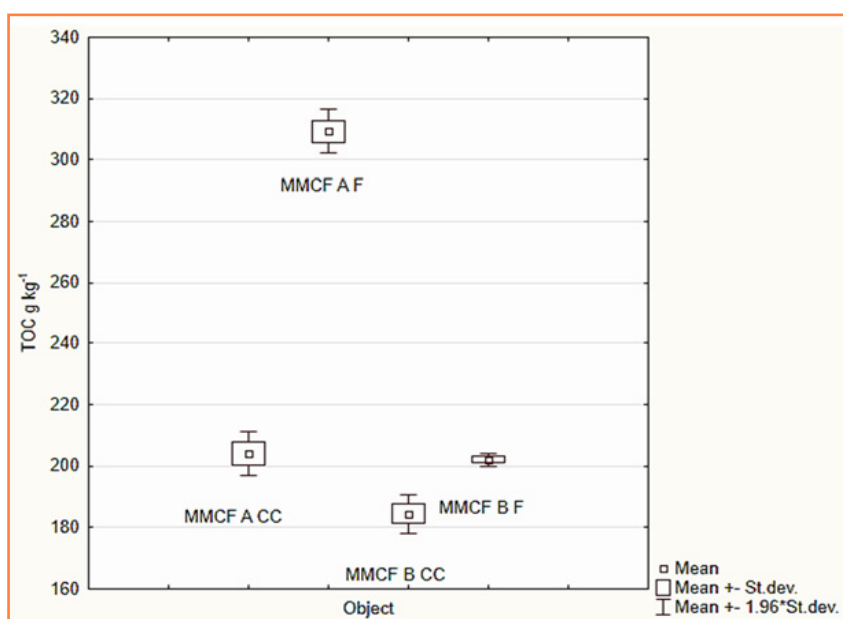
Figure 2 Total organic carbon (TOC) in Oa horizon of the soils under mountain mixed coniferous forest: undisturbed (MMCF F) and after clear-cutting (MMCF CC) A – Zmijowiec range, B – Bialskie Mts
