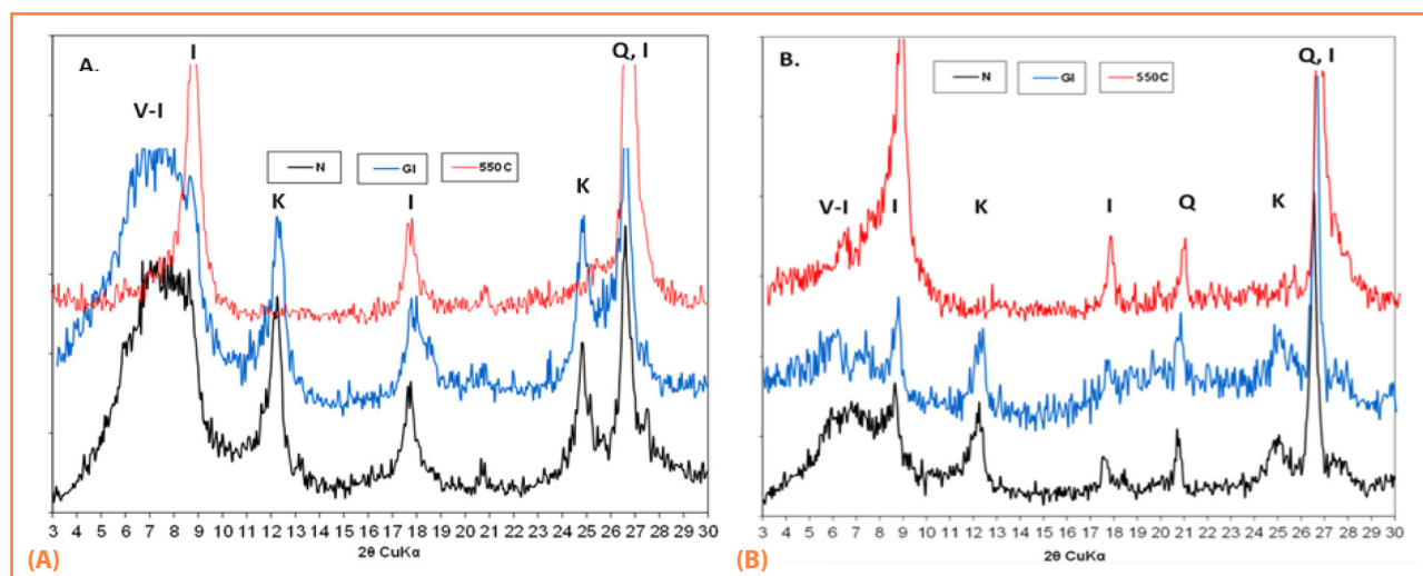
Figure 5 XRD patterns of clay fraction (<2 µm) in MMCF A CC object: (A) A horizon, (B) BC horizon Symbols for sample pretreatments: N – natural air-dried; GI – saturated with ethylene glycol, 550 °C – heated at 550 °C for 2 hours. Mineral designations: V-I – vermiculite-illite, I – illite, K – kaolinite, Q – quartz, V – vermiculite
