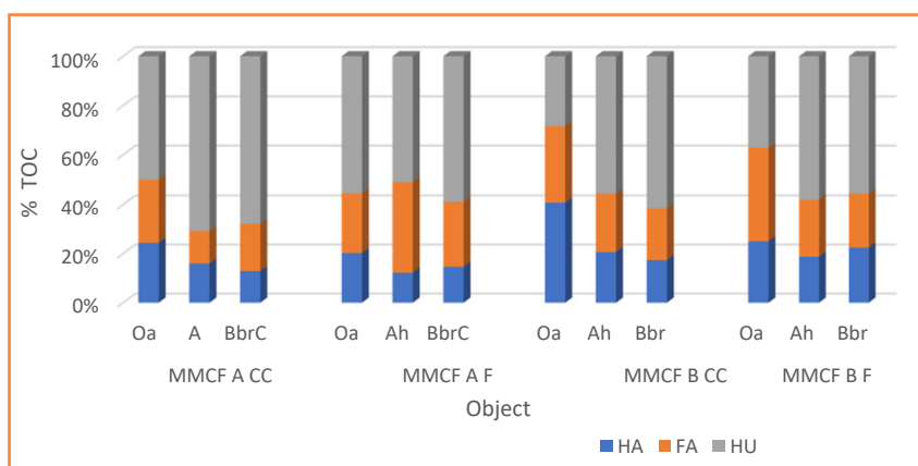
Figure 3 The content of humic (HA), fulvic acids (FA), and humins (HU) in soil profile under mountain mixed forest without harvesting practice (F) and after clear-cutting (CC) in the East Sudety Mountains
