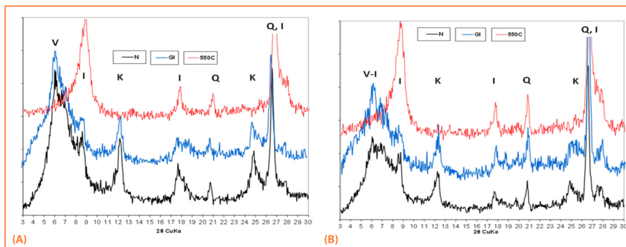
Figure 6 XRD patterns of clay fraction (<2 μm) in MMCF A F object: A) A horizon, B) BC horizon. Symbols for sample pretreatments: N – natural air-dried; GI – saturated with ethylene glycol, 550 °C – heated at 550 °C for 2 hours. Mineral designations: V-I – vermiculite-illite, I – illite, K – kaolinite, Q – quartz, V – vermiculite
