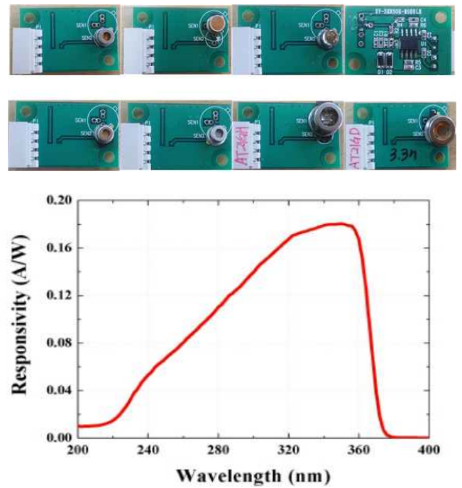
Figure 3 PCB and Response curve of UV sensor.
