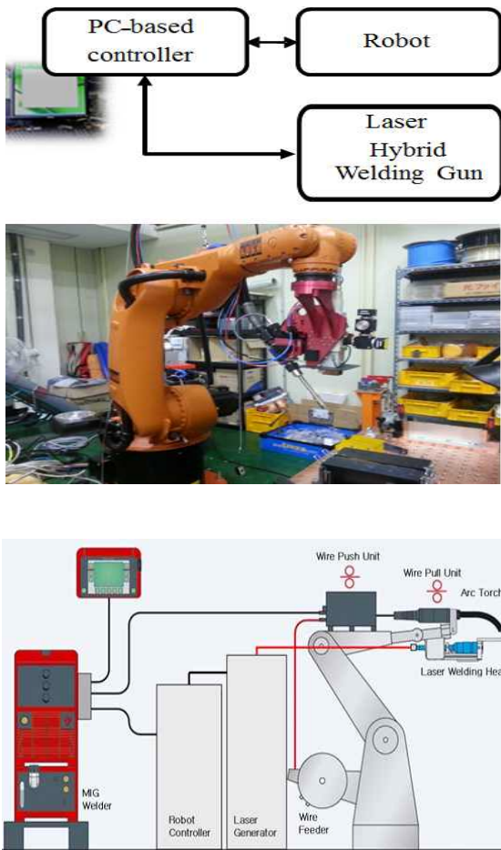
Figure 1 The robot-based laser hybrid welding system: control block diagram (top), photo (middle), and illustration (bottom).
