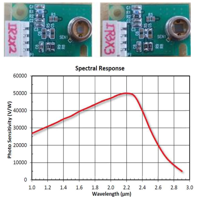
Figure 4 PCB and Response curve of IR sensor.
