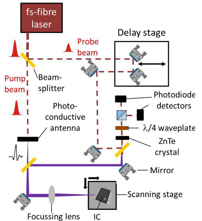
Figure 1. Schematic of the THz measurement system with corresponding beam paths. Dashed lines show the near infrared femtosecond fibre laser. Solid line represents the THz path.
