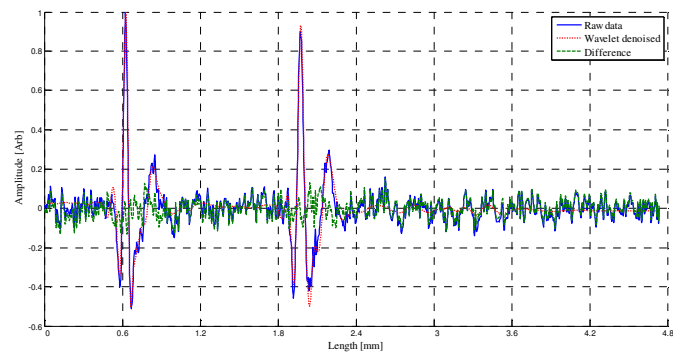
Figure 3. Raw data input in blue, the Wavelet denoised version in red and the difference of both in green.
