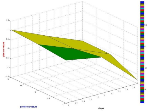
Figure 1. 3D surface mesh-grid of covariant unit terrain attributes
