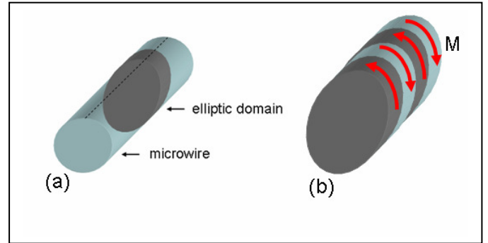
Figure 1. (a) Elliptic domain in microwire; (b) Direction of magnetization in elliptic multi-domains structure.
