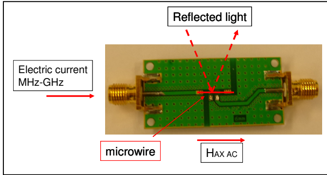
Figure 2. Sample cell.
