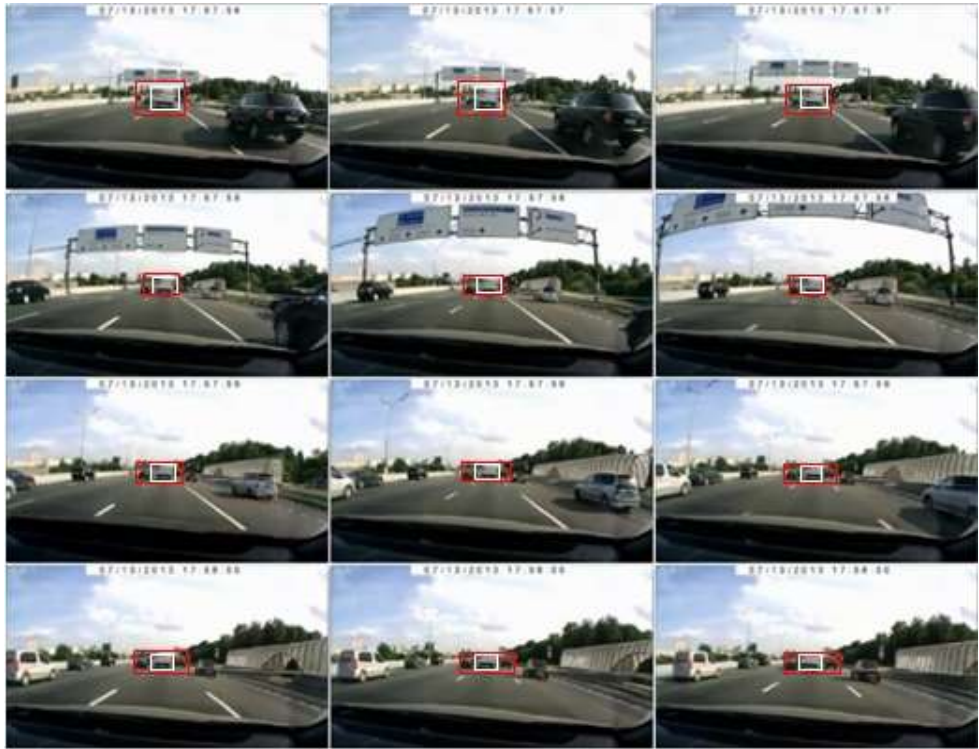
Figure 11. Detecting and tracking running truck in express way with dynamic noisy background caused by similar cars (white squares stand for N-SVDD, red squares stand for Mean-Shift)
