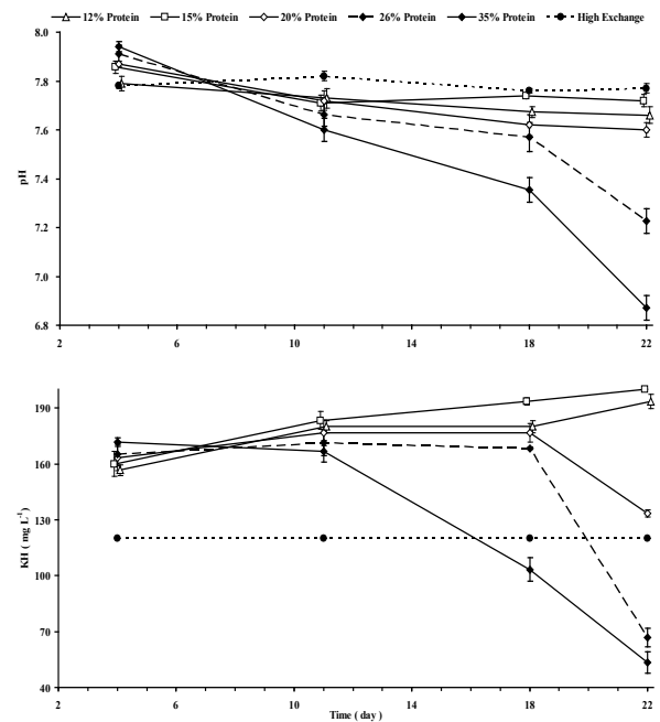
Fig. 3. Effects of dietary protein on pH and total alkalinity (KH) for zero exchange in 23 day growth trial with juvenile shrimp stocked at 6.21 \text{ g} \pm 0.22 \text{ (SD)} . For zero exchange, values are means ( \pm S.E ) of three replicate tanks per sampling time at each protein level. The high exchange represents combined observations of all protein levels at high water exchange ( n = 5 ).
