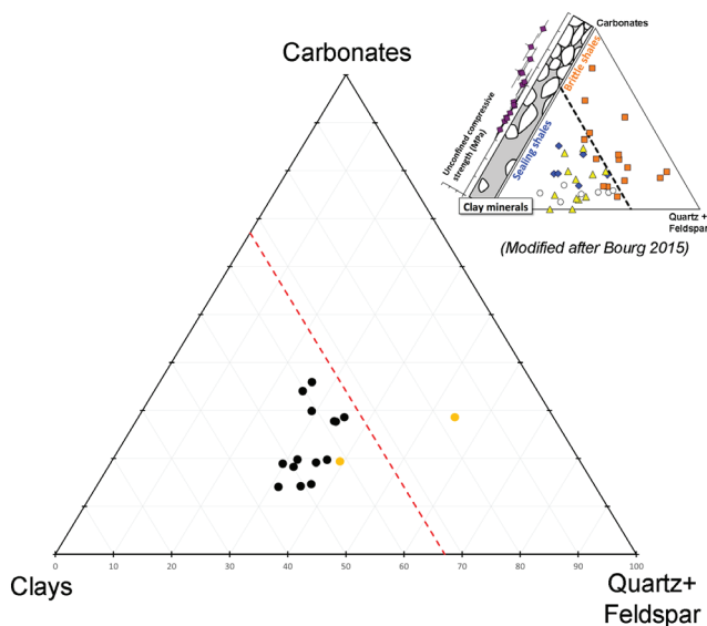
Figure 11: Ternary diagram of the whole-rock XRD analysis of selected samples from the cored intervals of Bockfließ Formation in Matzen 269 well. Black dots indicate lagoon facies, whereas yellow dots represent Washover Fan facies. Dashed line represents the 33 %-clay threshold after Bourg (2015).
