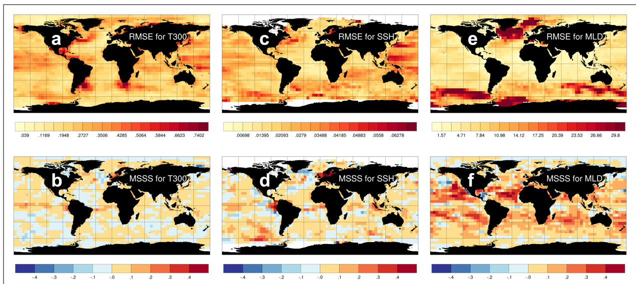
Figure 6 The upper row: the global maps of RMSE for yearly T300 anomalies (unit: °C), SSH anomalies (unit: meter), and MLD anomalies (unit: meter) in the filter analysis (reference). The lower row: the global map of MSSS for yearly T300, SSH, and MLD anomalies. In this experiment, SST observation error variance is inflated by a factor of four.
