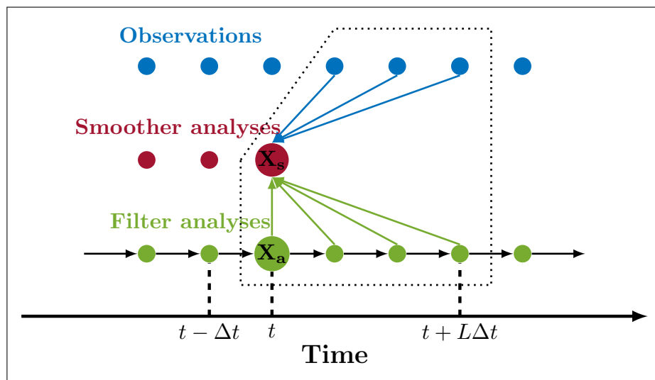
Figure 1 Schematic of the offline EnKS. The green dots represent the filter analysis after a model integration of \Delta t schematized by the black arrows. The blue dots depict the observations, and the red dots represent the smoother analyses of the offline EnKS. The dotted shape contains ‘future’ observations and filter analyses from t to t + L\Delta t to generate the smoother analysis \mathbf{X}_s at t , in which the blue and green arrows are information flows.
