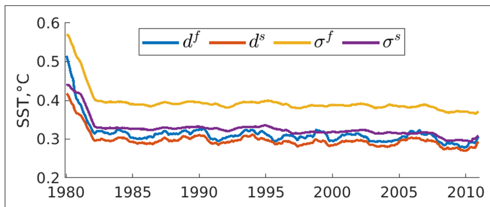
Figure 4 Global assimilation statistics for monthly SST (i.e., assimilated quantity): RMSE for the filter analysis (blue line), RMSE for the smoother analysis (red line), combined error for the filter analysis (orange line), and combined error for the smoother analysis (purple line). The time series is smoothed with a time window of 12 months.
