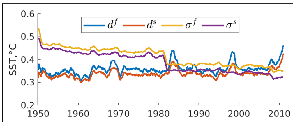
Figure 7 Global assimilation statistics for monthly SST anomalies (i.e., assimilated quantity): RMSE for the filter analysis (blue line), RMSE for the smoother analysis (red line), combined error for the filter analysis (orange line), and combined error for the smoother analysis (purple line). In this experiment, \gamma = 0.1 , and the observation error variance is inflated by four. The time series is smoothed with a time window of 12 months.
