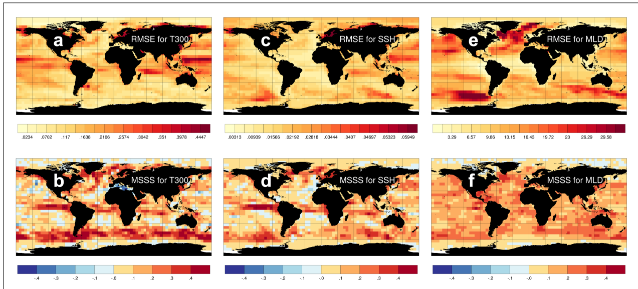
Figure 3 The upper row: the global maps of RMSE for monthly T300 (unit: °C), SSH (unit: meter), and MLD (unit: meter) in the filter analysis (reference). The lower row: the global map of MSSS for monthly T300, SSH, and MLD.
