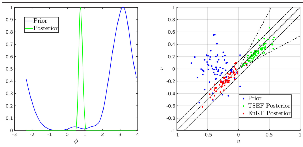
Figure 2 Left: The prior (blue) and posterior (green) pdfs of angle \phi . Both are normalized to have unit maximum height so their shapes can be compared more easily. Right: A prior ensemble of wind vectors (blue), together with the posterior ensemble of wind vectors produced by the probability integral transform approach (green) and the EnKF approach (red). The solid black line is in the direction of the observed wind; the dotted black line is opposite to the direction of the observed wind; the dashed lines enclose the directions with nonzero likelihood; and the dash-dotted lines enclose the 95% confidence interval associated with the EnKF observation model.
