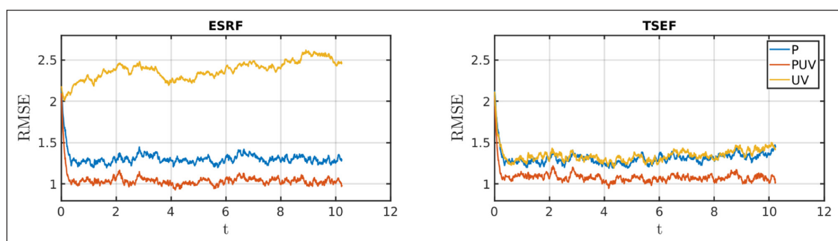
Figure 5 Time series of RMSE for the ESRF (left) and TSEF (right) filters with random observation locations. In the legend, P denotes experiments assimilating only observations of pressure, PUV denotes experiments assimilating observations of pressure and wind direction, and UV denotes experiments assimilating only observations of wind direction. The climatological standard deviation of vorticity is 2.17, for reference.
