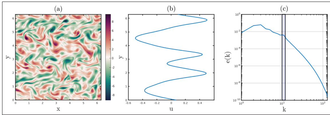
Figure 3 Properties of the reference experiment. (a) A snapshot of vorticity \omega . (b) The time-mean and zonal-mean velocity profile. (c) The kinetic energy spectrum; the range of forcing wavenumbers is shaded. All variables are nondimensional.
