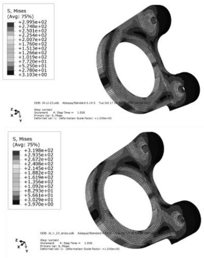
Fig. 7 von Mises stress for isotropic (up) and anisotropic (down) analysis
