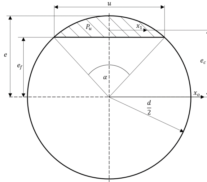
Fig. 4. Cross section model with fatigue failure used for consideration.
