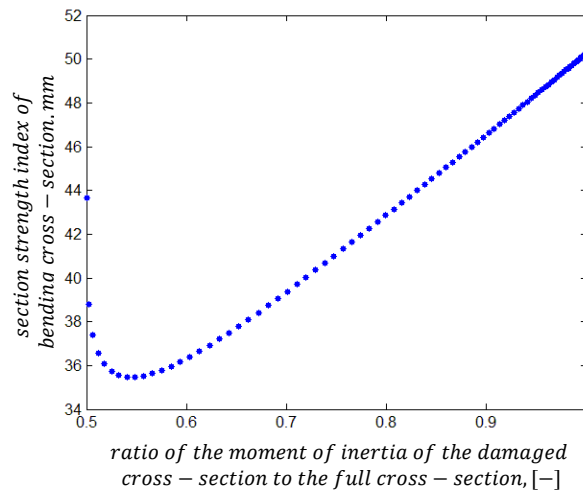
Fig. 6. Variation of the section strength index on bending with respect to the moment of inertia of the bending cross section
