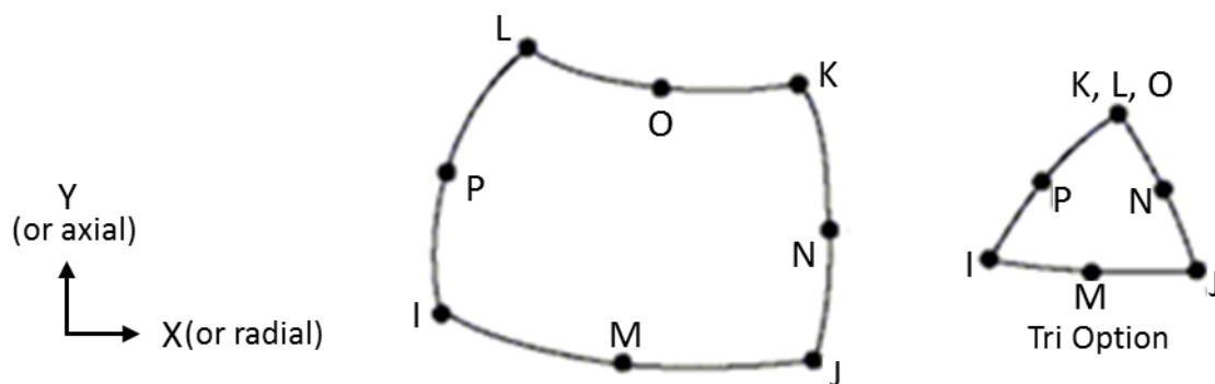
Fig. 2 Geometry of the 2-D elements PLANE183 and PLANE223 [3]
