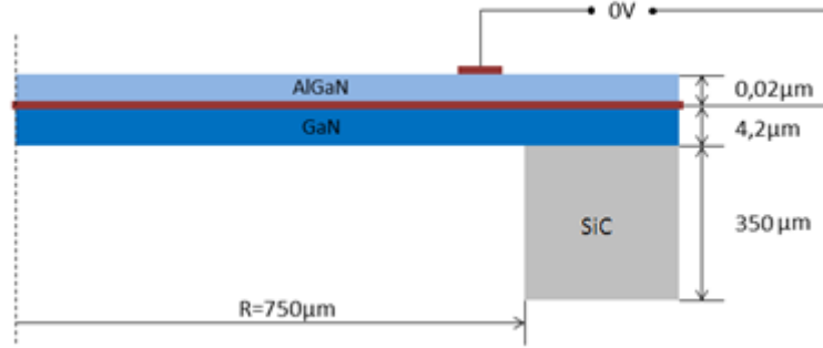
Fig. 1 Dimensions of the equivalent model of the membrane
