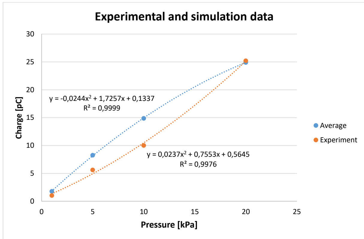
Fig. 6 Graphical representation of the average values (simulated) and experimental results
