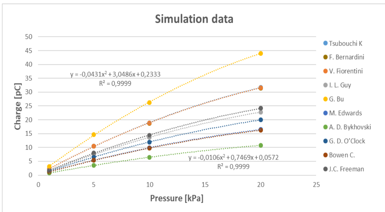
Fig. 5 Graphical representation of the simulation results
