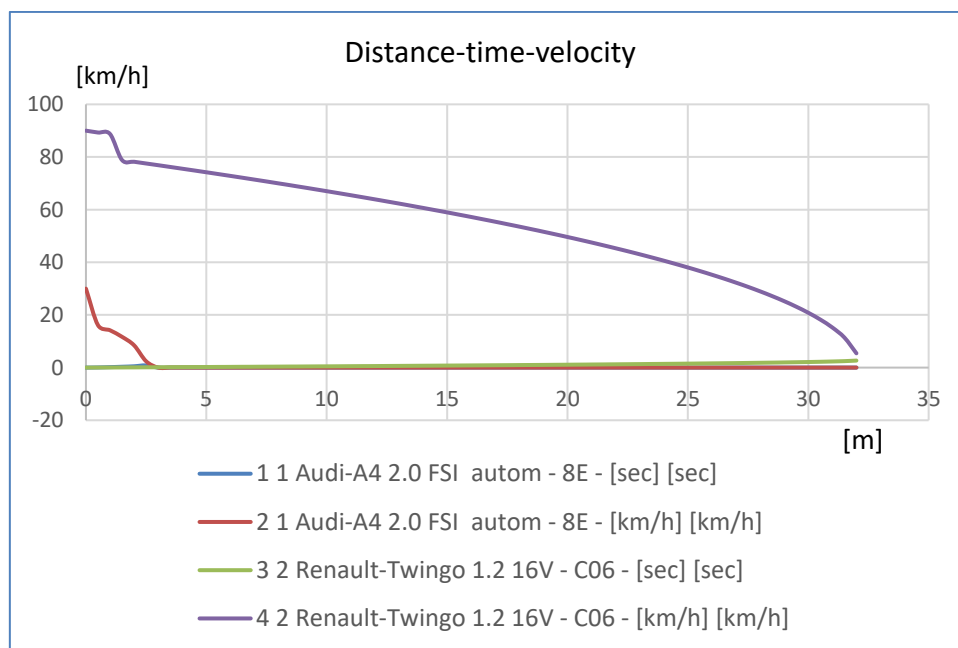
Diagram 1. Report distance – time – velocity
