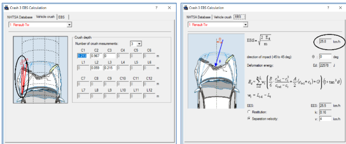
Fig. 5 PC Crash calculation of lost velocity in deformation of “Renault”
