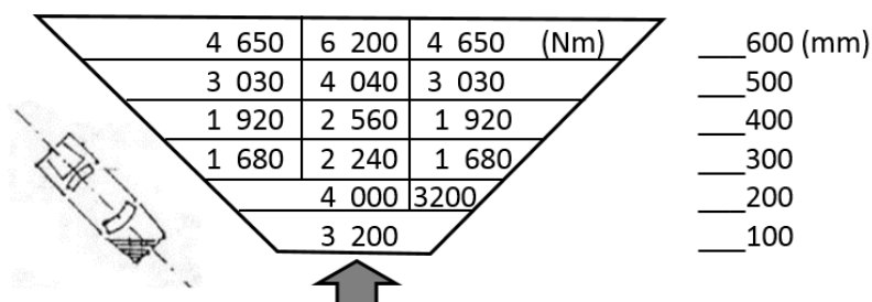
Fig. 8 Energy deformation for angular deformations of vehicle
