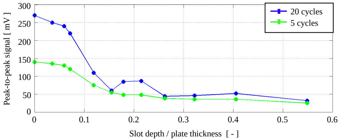
Fig.16 Transmission method: peak-to-peak amplitudes as a function of h_p/2b , for a 20-cycle impulse and a 5-cycle impulse
