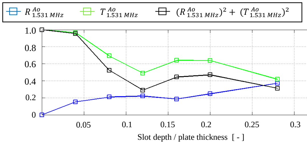
Fig.8 Dispersion coefficient trend for f_0 = 1.531 MHz, 20-cycle Hann modulation
