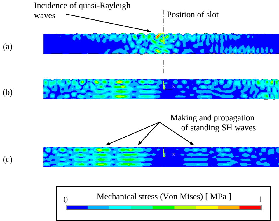
Fig.9 Interaction of a quasi-Rayleigh wave ( f_0 = 1.531 MHz, 20 cycles) and a perpendicular slot ( h_p = 0.838 mm): (a) time: 45 \mu s; (b) time: 55 \mu s; (c) time: 60 \mu s
