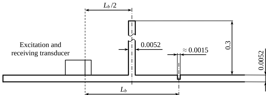
Fig.12 Diagram of sample dimensions and transducer location for the reflection method
