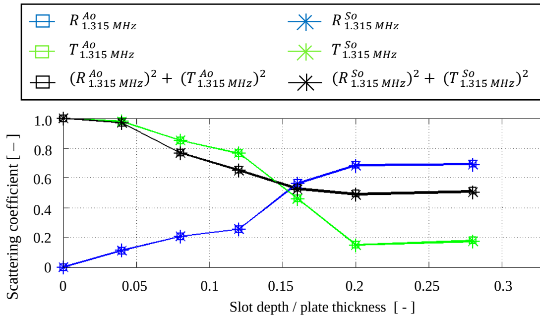
Fig.7 Dispersion coefficient trend for the wave frequency ( f_0 ) of 1.315 MHz, 5-cycle Hann modulation
