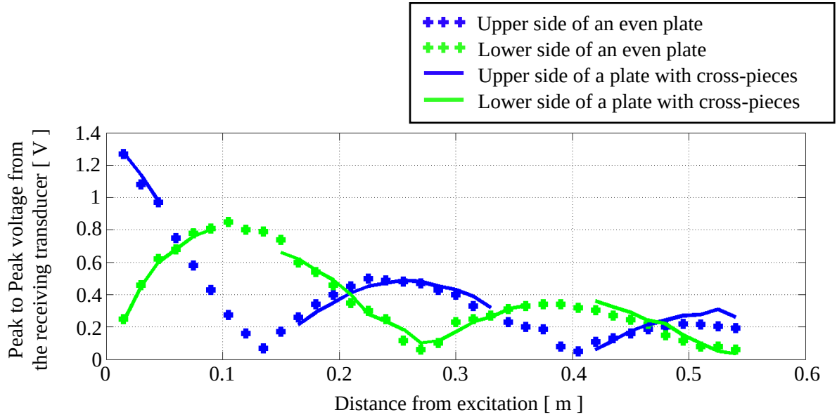
Fig. 5: Comparison of the peak-to-peak amplitudes of waves for an even plate and a cross-piece plate of the same thickness ( f = 1.55 MHz; 20-cycle Hann modulation; L_b \approx 0.2774 m); the thickness of cross-pieces is the same as the plate thickness and the distances of the cross-pieces from the transducer are 0.135 m and 0.405 m.
