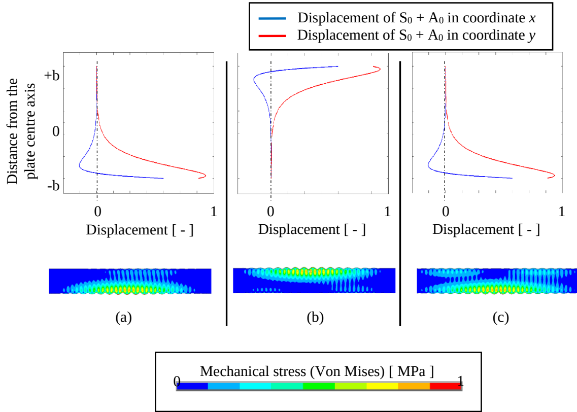
Fig. 4: Representation of the resulting S_0 + A_0 modes and of (von Mises) stresses at FEM model (simulation of quasi-Rayleigh wave propagation) at distance x from the starting point of propagation: (a) x = 0 m; (b) x = L_b/2 ; (c) x = L_b
