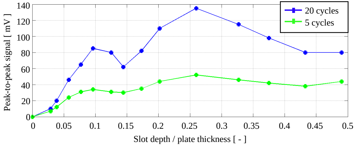
Fig.13 Reflection method: peak-to-peak amplitudes as a function of slot depth / plate thickness ratio for a 20-cycle impulse and a 5-cycle impulse
