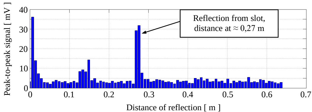
Fig.14 Peak-to-peak amplitudes as a function of the propagation distance of waves (5-cycle impulse)
