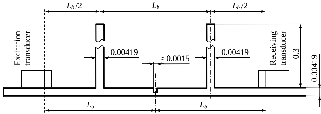
Fig.15 Diagram of sample sizes and transducer locations for the transmission method
