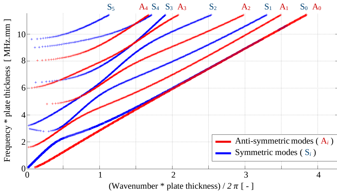
Fig. 2 Dispersion curves of real wavenumbers for steel properties
