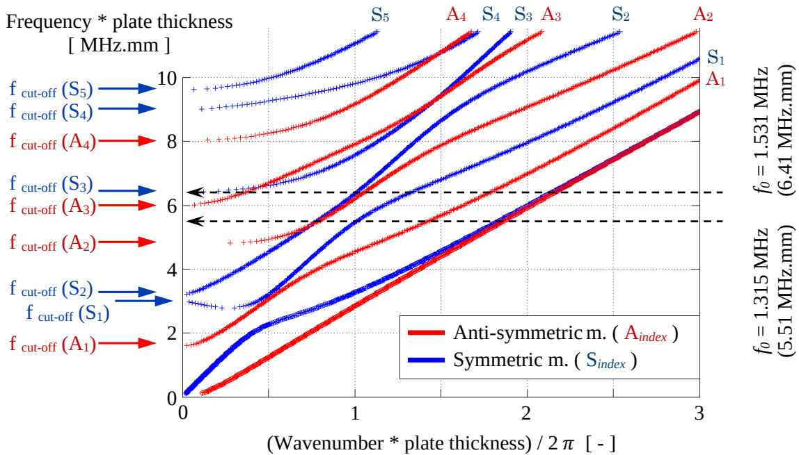
Fig.10 Cut-off frequency values and simulation values marked in the dispersion curve
