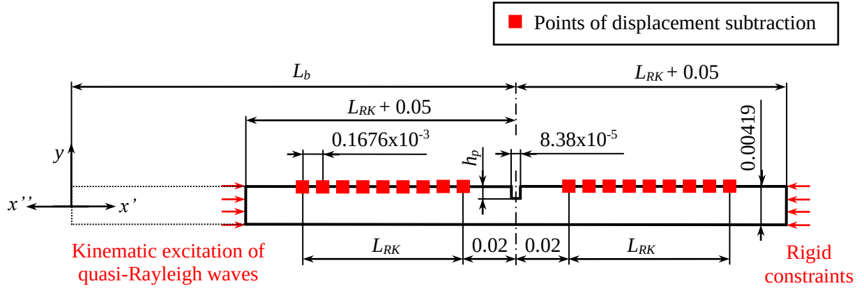
Fig.6 FEM simulation model diagram (the x' axis reflects the subtraction of incident waves and transmitted waves; the x'' axis reflects the subtraction of reflected waves); dimensions are expressed in metres.
