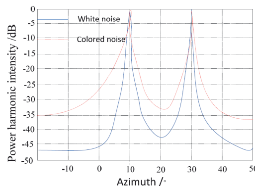
Fig. 4. Location search results after suppression of surge interference with using the proposed method.
