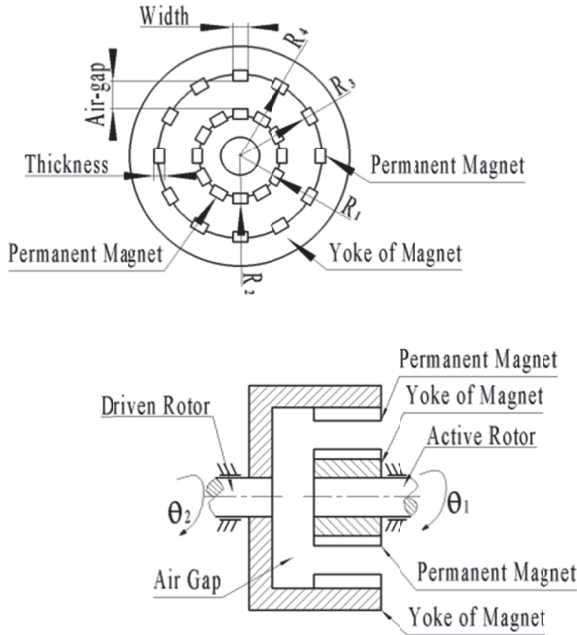
Fig. 1. Magnetic Coupling Model
