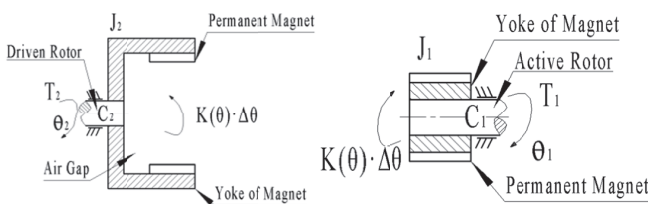
Fig. 2. Force Distribution.
