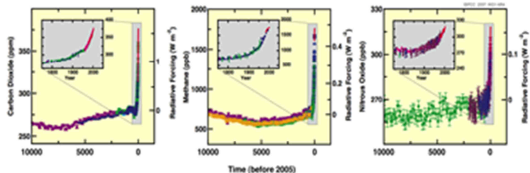
Changes in Greenhouse Gases from ice-core and Modern Data
