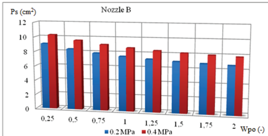
Figure 8. Total covering ( P_s ) of the sprayed objects depending on the W_{po} with pressure liquid 0.2 and 0.4 MPa for nozzle B
