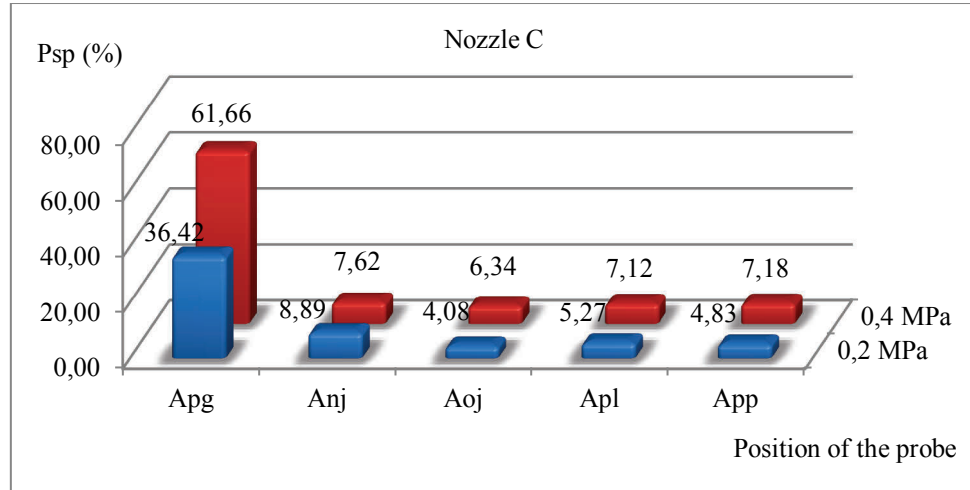
Figure 3. Degree of coverage ( P_{sp} ) of probes for nozzle C at the pressure of 0.2 and 0.4 MPa
