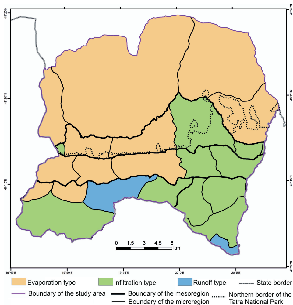
Fig. 9. Variation in the dominance of hydrotope types in the study area.
