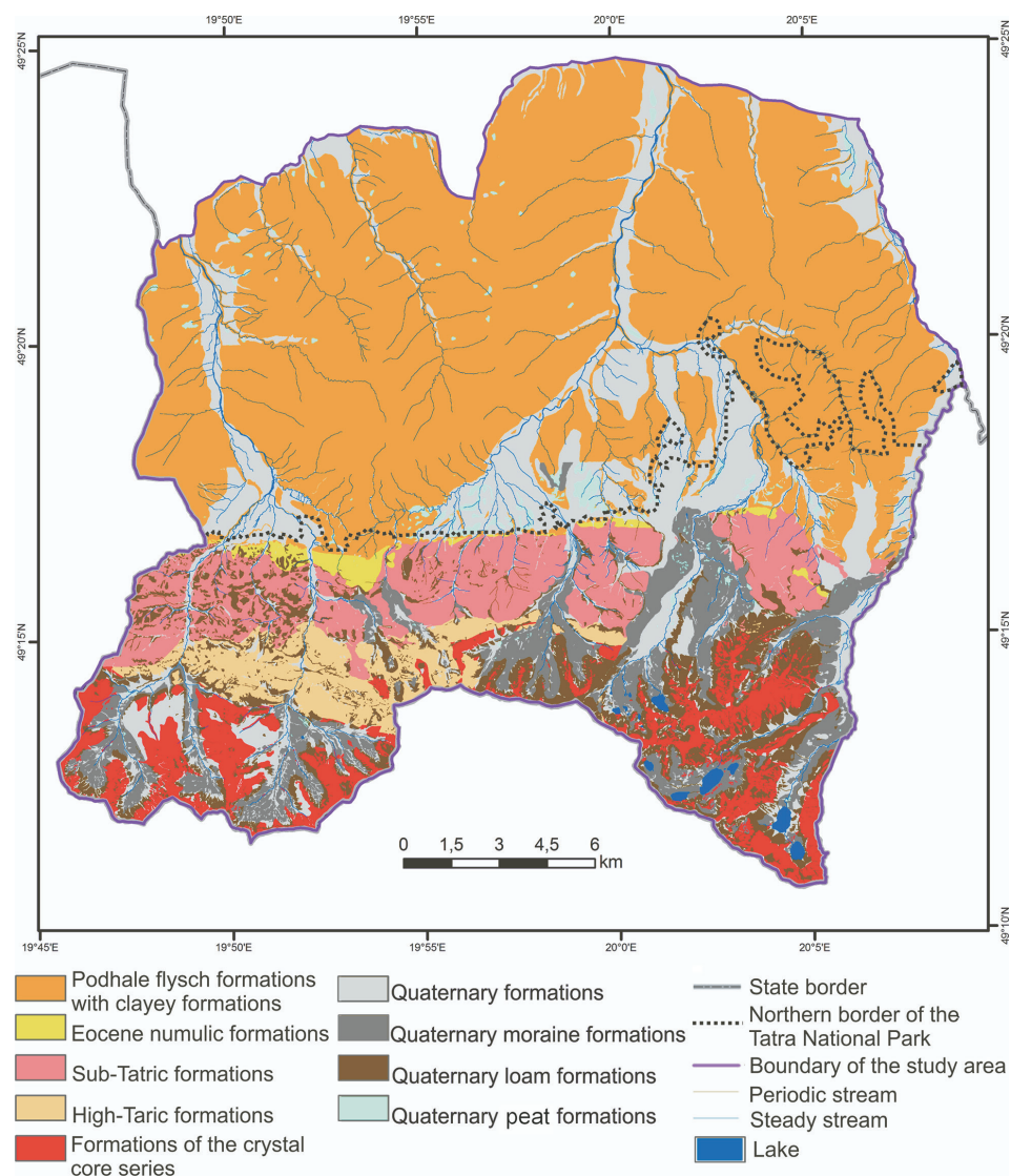
Fig. 2. Geological structure of the study area based on Guzik, Guzik (1958), Guzik et al. (1958, 1959, 1975), Michalik (1958), Guzik (1959a, b), Michalik, Guzik (1959a, b), Detailed Geological Map of Poland (1975, 1976), Guzik, Jaczynowska (1978), Bac-Moszaszwili et al. (1979), Sokołowski, Jaczynowska (1979a, b, 1980), Jaczynowska (1980) and Małecka (1982).
