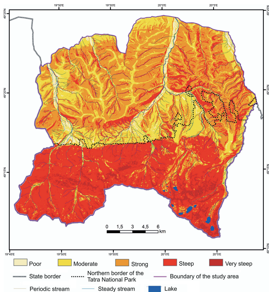
Fig. 5. Slope gradients in the study area based on Digital Elevation Model (GUGiK 2009).
