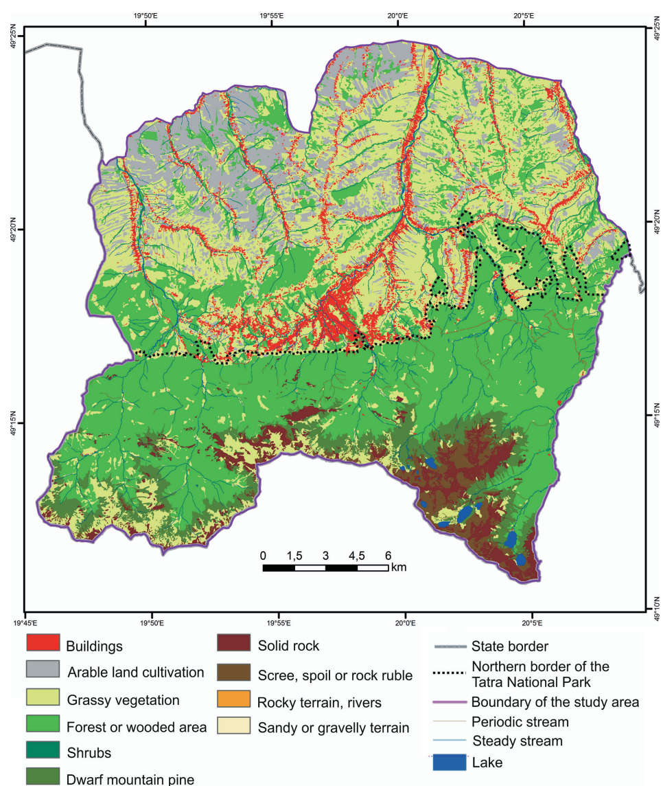
Fig. 4. Land cover of the study area based on Regulation of the Minister of Internal Affairs and Administration of 17 November 2011 on the database of topographic objects and the database of general geographic objects, as well as standard cartographic studies (2011), Database of Topographical Objects, 1:10,000, (BDOT10k) (GUGiK 2013).
