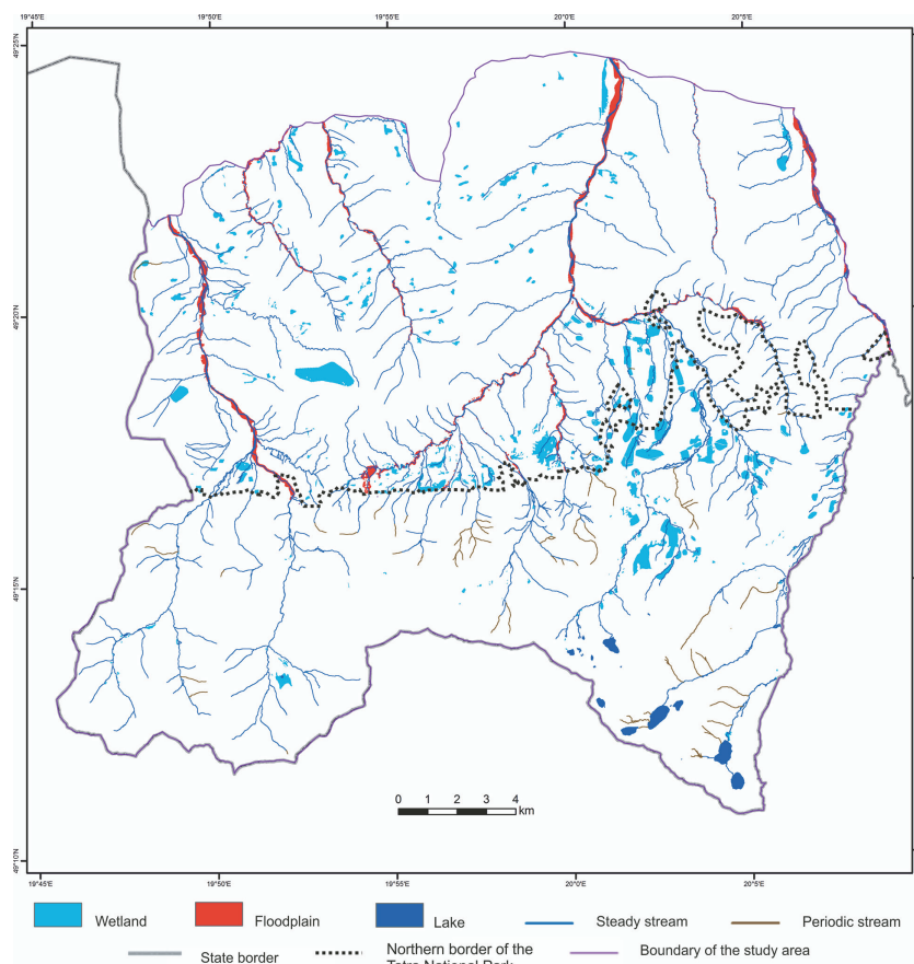
Fig. 6. Wetlands, permanent, periodic and areas flooded in the study area based on the Hydrographic Map of Poland (2006).
