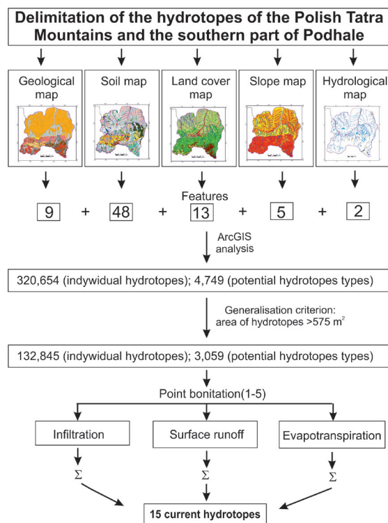
Fig. 7. Flowchart for the delimitation of hydrotope type.
