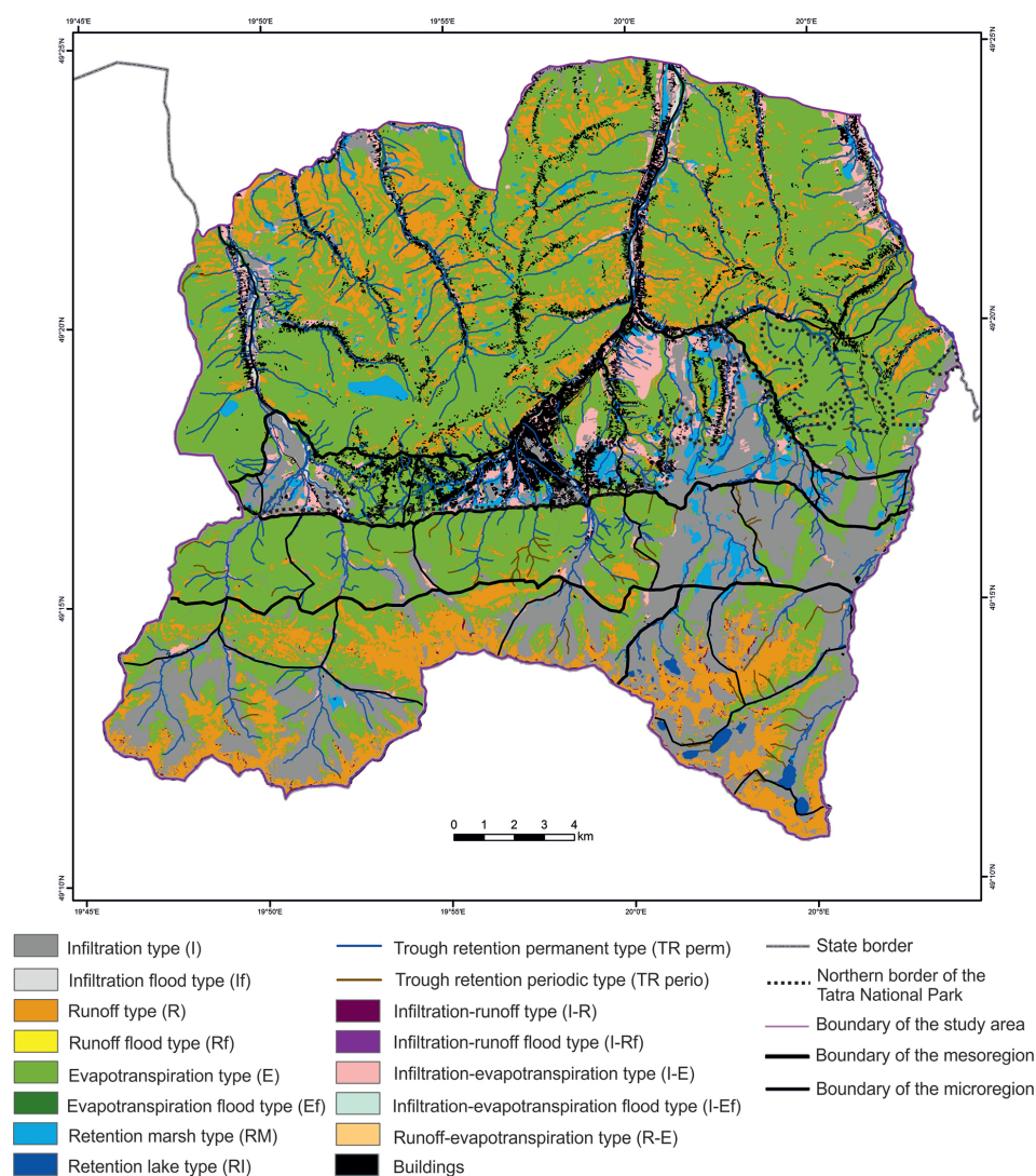
Fig. 8. Spatial variation of hydrotope types in the study area.
