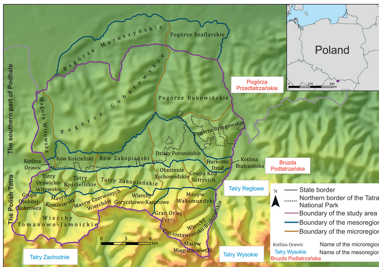
Fig. 1. Physical-geographical division of the study area (Balon et al. 2015, Krąż, Wójcik 2015, Jodłowski et al. 2021a, b) model: ASTER Global DEM (n.d.)*. In the study, the names of lower-level physiogeographic units (microregions and mesoregions) are provided in Polish. The names commonly known and used in the international literature (Carpathians, Tatra Mountains) are written in English.
