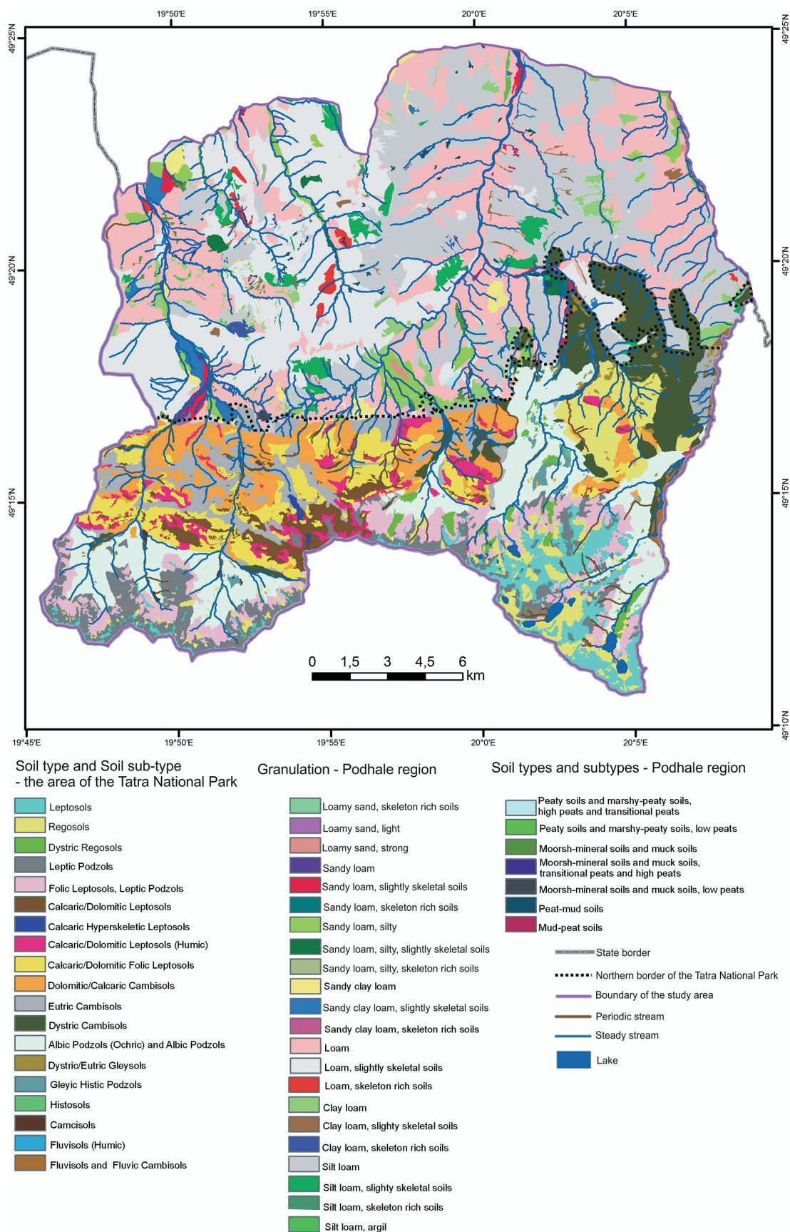
Fig. 3. Soil cover of the study area based on Soil and Agricultural Map (1963–1980) and Skiba (2002); classification of soil types based on the IUSS Working Group WRB (2022).
