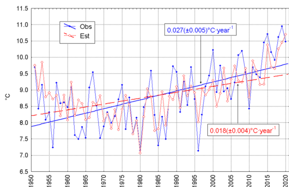
Fig. 5. The course of the observed mean annual air temperature ( ^{\circ}\text{C} ) in Kraków (Obs) and the estimated air temperature based on sunshine duration (Est) from 1951 to 2020. The trend values are marked in boxes (with the standard error of estimation values in parentheses).
