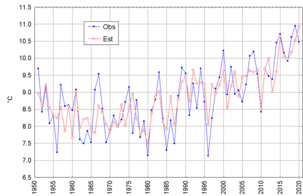
Fig. 9. The course of the observed annual average air temperature ( ^{\circ}\text{C} ) in Kraków (Obs) and the estimated (Est) temperature based on the course of three variables: sunshine duration (SD), North Atlantic Oscillation (NAO), and \Delta F from 1951 to 2020.
