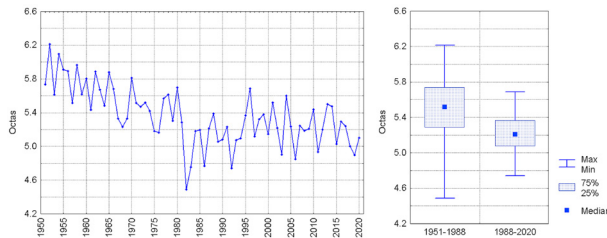
Fig. 3. Course of annual cloudiness values (oktas) in Kraków in the period 1951–2020, and ranges of its variability in periods 1951–1988 and 1988–2020.
