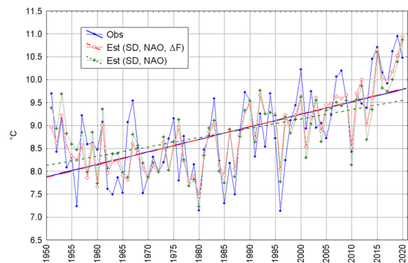
Fig. 10. Course of the observed average annual air temperature ( ^{\circ}\text{C} ) in Kraków (Obs) and the estimated temperature (Est) based on the course of two variables sunshine duration (SD) and North Atlantic Oscillation (NAO) and three variables (SD, NAO, and \Delta F ) in the years 1951–2020. Trend lines are marked. The differences between the observed temperature trend and the estimated temperature trend based on three variables are so small ( 0.001^{\circ}\text{C} \cdot \text{year}^{-1} ) that they overlap in the graphical representation
