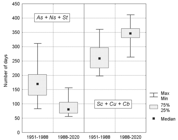
Fig. 4. Ranges of variability in the number of days with observations of frontal clouds ( As , Ns , St ) and clouds occurring in unstable weather conditions in Kraków during the periods 1951–1988 and 1988–2020.
