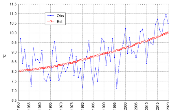
Fig. 8. Course of the observed mean annual air temperature ( ^{\circ}\text{C} ) in Kraków (Obs) and the estimated (Est) from the course of radiative forcing in the years 1951–2020.
