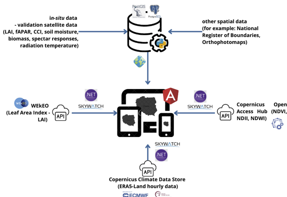
Fig. 4. Diagram of proceedings in the development of the GRASSAT application.
