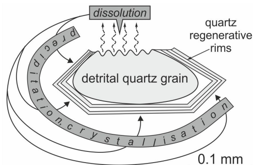
Fig. 4. Sketch of the formation of freshwater quartzite sandstones in a palaeosol environment (modified from Górniak et al., 1996). Note where silica dissolves and precipitates.
