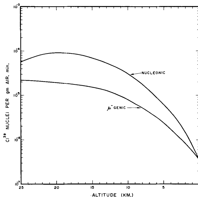
FIG. 5. Calculated rates of production of \text{Cl}^{39} due to secondary cosmic ray nucleons and mu-mesons at \lambda = 20^\circ are shown as a function of altitude.
