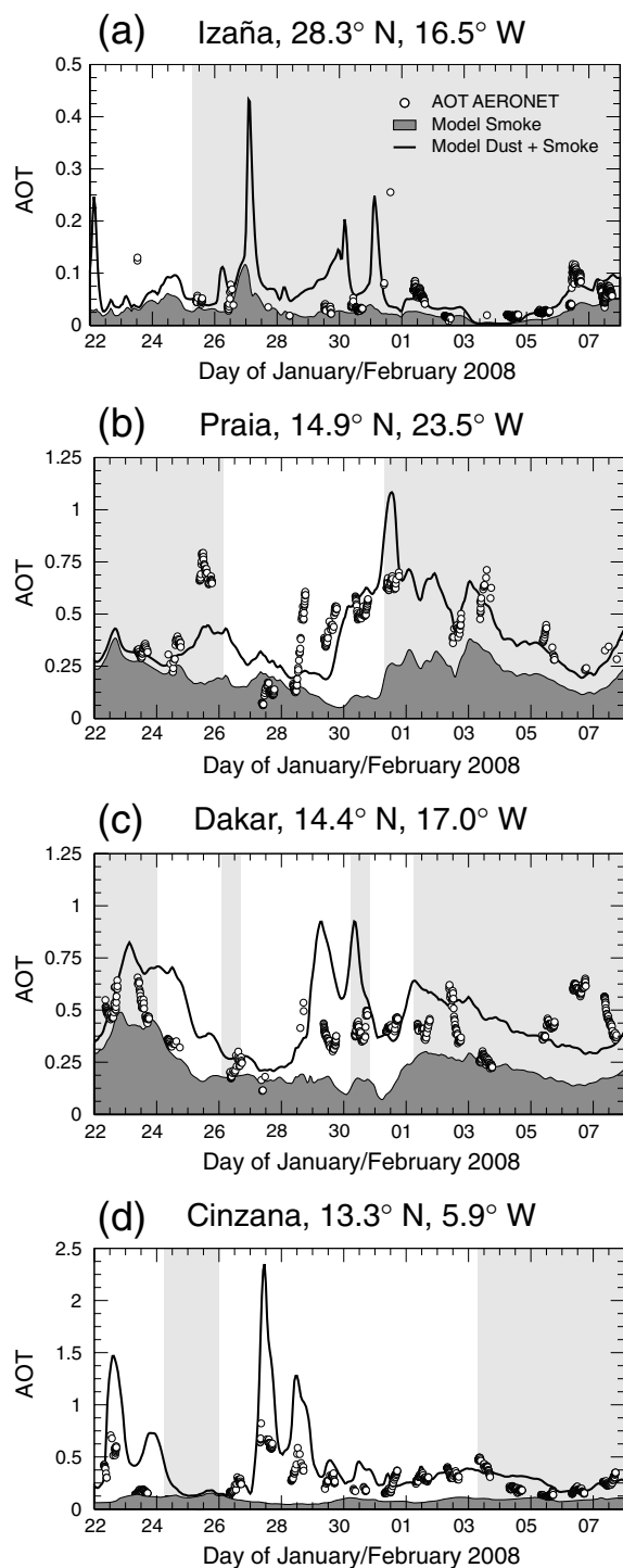
Fig. 7. Aerosol optical thickness (440 nm) at Izaña/Tenerife, Praia/Santiago, Dakar and Cinzana on 22 January–7 February 2008. Compared are sun photometer measurements provided by AERONET (black circles) and values of optical thickness of modelled smoke (dark grey shaded area) and the mixed plume of dust and smoke (solid black line). Grey shaded areas denote the days, on which the Ångström exponent ( \alpha ) from AERONET measurements indicates a smoke-dominated aerosol layer ( \alpha > 0.3 ).
