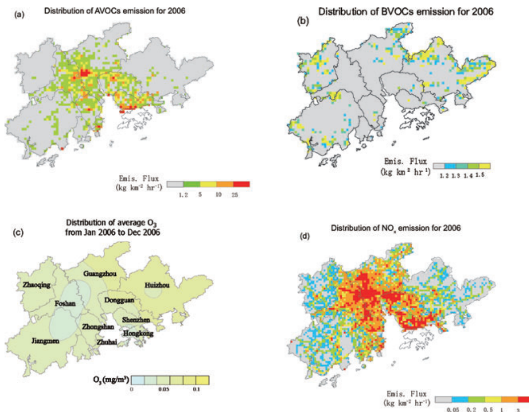
Fig. 8. (a) AVOC emission flux, (b) BVOC emission flux, (c) annual average O_3 concentration and (d) anthropogenic NO_x emission flux for 2006. Source: (a,d) From Zheng et al. (2009) and (c) from http://www-app.gdepb.gov.cn/EQPublish/raqi.aspx .
