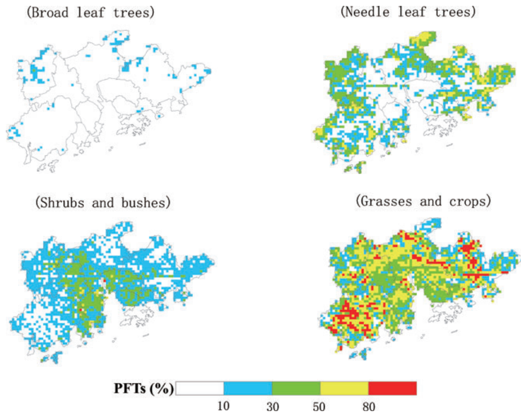
Fig. 6. Plant functional types (PFTs) distribution with MODIS data.
