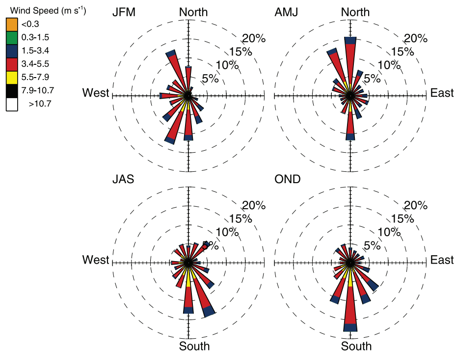
Fig. 3. Wind rose for winter, spring, summer, and fall. Based on data collected 4 m above the ground at the ARM Climate Research Facility.
