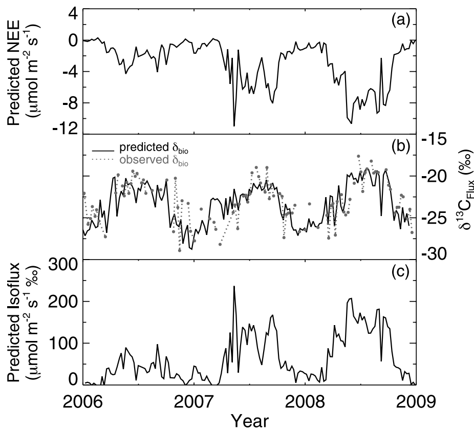
Fig. 7. Estimate of isoflux using observed weekly average wind direction, ISOLSM predictions, and Keeling plot results. (a) Average predicted NEE upwind of the observation tower; (b) the \delta_{\text{bio}} values observed at the tower (dashed line) and predicted by ISOLSM for the SGP quadrant upwind of the observation tower (solid line); and (c) isoflux calculated as \text{NEE} \times \delta_{\text{bio}} for each time point using predicted NEE and \delta_{\text{bio}} . Positive isoflux means NEE enriches atmospheric \delta_{\text{atm}} .
