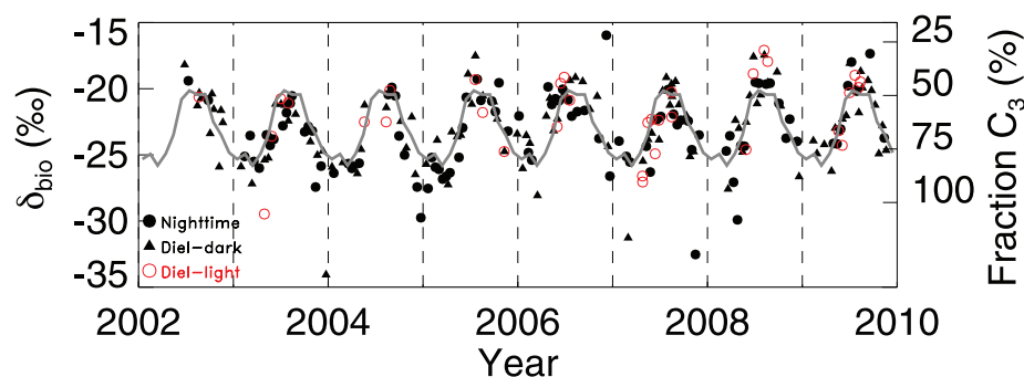
Fig. 6. Time series of the isotopic signature of carbon exchange ( \delta_{\text{bio}} ) at SGP. Only data with intercept SE < 1.5\text{‰} are shown. The nighttime Keeling plot intercepts (solid circles, n = 97 ) were generated with 16 flasks at four heights overnight. The diel-dark (solid triangles; n = 116 ) and diel-light (open circle, N = 33 ) intercepts use flasks from 2 and 60 m collected over a diurnal cycle. There were few day-light Keeling plot intercepts with SE < 1.5\text{‰} between November and February because photosynthetic fluxes and atmospheric ^{13}\text{CO}_2 gradients were too small. The grey line shows the ensemble monthly means for all these data; there were 88 monthly averages for the 96-month period and the line shows the 8-yr ensemble average value for each month (for example, the average of all eight October months in the record; see Table 2).
