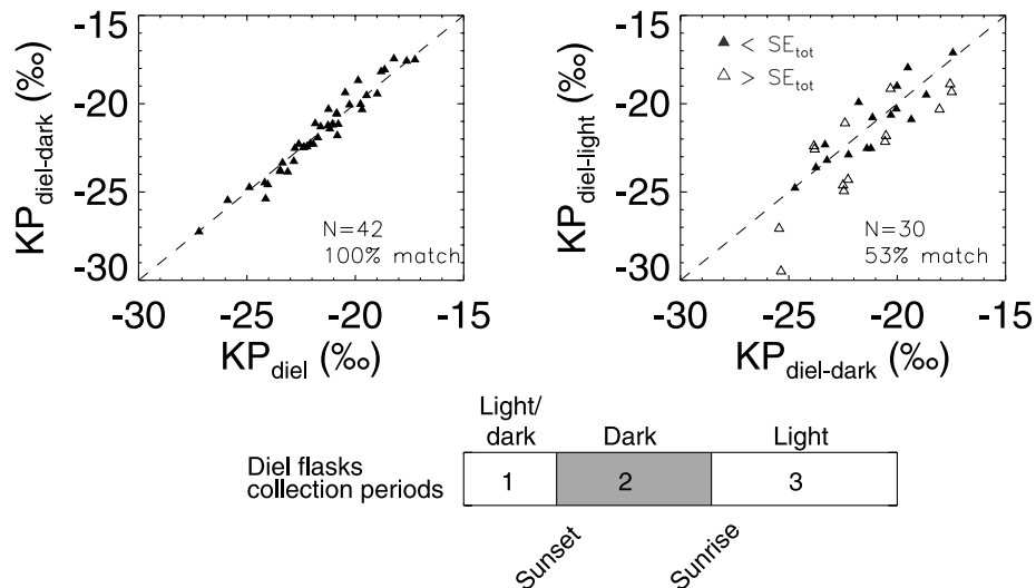
Fig. 5. The 21 h diel sampling can be divided into three periods: (1) the late afternoon of the first day, (2) the dark period between sunset and sunrise and (3) the morning to afternoon of the following day. The left panel compares the Keeling plot intercept generated by the diel-dark flasks (period 2) with that from the whole diel period (period 123). These two \delta_{\text{bio}} values (i.e. Keeling plot intercepts) matched in 100% of the cases, meaning the difference between the diel and diel-dark-only intercepts was less than the SE of the two values. The right panel shows the relationship between diel-dark and diel-light (period 3) Keeling plot intercepts. The closed symbol indicates that the dark and light values matched; the open symbols indicate a larger difference relative to the SE. In both plots, data are shown only for Keeling plots with \text{SE} < 1.5\text{‰} ( N = 42 for dark (2); N = 30 for dark and light (3)). The symmetry of scatter around the dashed 1:1 line shows the lack of bias between either the whole diel versus diel-dark periods or the diel-dark versus diel-light periods. Flasks were collected every three hours at 2 and 60 m starting at 18:00 local time.
