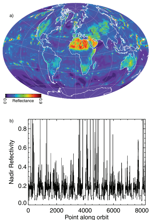
Fig. 2. Surface reflectance fraction used in the instrument performance simulations: (a) global and (b) sampled along the orbit track for one example day. Reflectance over land is obtained from the MODIS Band 6 16-d composite BRDF-adjusted nadir reflectance product. Missing data are filled with values of 0.2. Over water, Fresnel reflectance is calculated at nadir using 10-m wind speed from the meteorological analysis. Reflectance over ice that is not available from MODIS (e.g. in the polar dark) is assumed to be 0.1 (Warren, 1982). Ice cover extent is determined from the GEOS-4 analysis.
