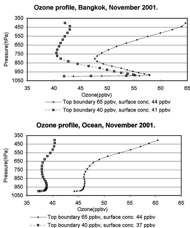
Fig. 8. Modelled vertical ozone profiles showing the dependence of surface ozone on upper boundary values. (A) Bangkok (13.75°N, 100.5°E), (B) ocean (15°N, 115°E).
