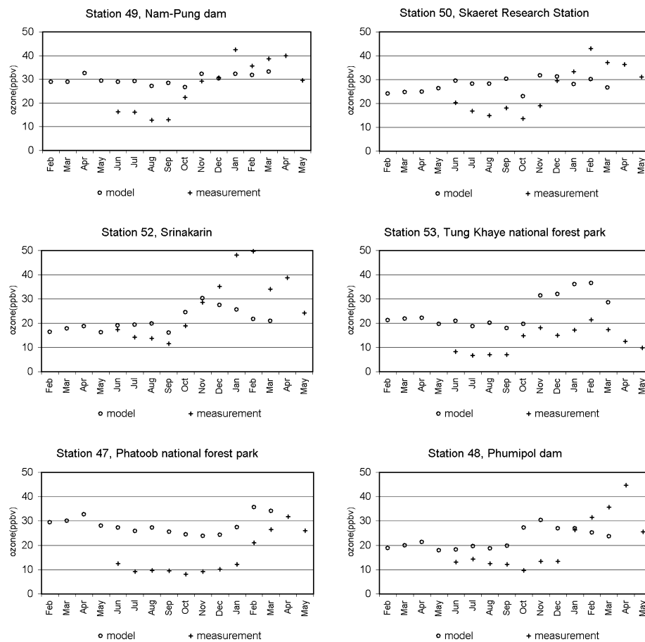
Fig. 3. Seasonal variation of ozone at remote stations in Thailand. Measured data from Iverfeldt et al. (2003).
