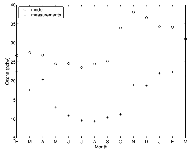
Fig. 2. Monthly means of ozone averaged over 36 non-remote stations from February 2001 to March 2002.
