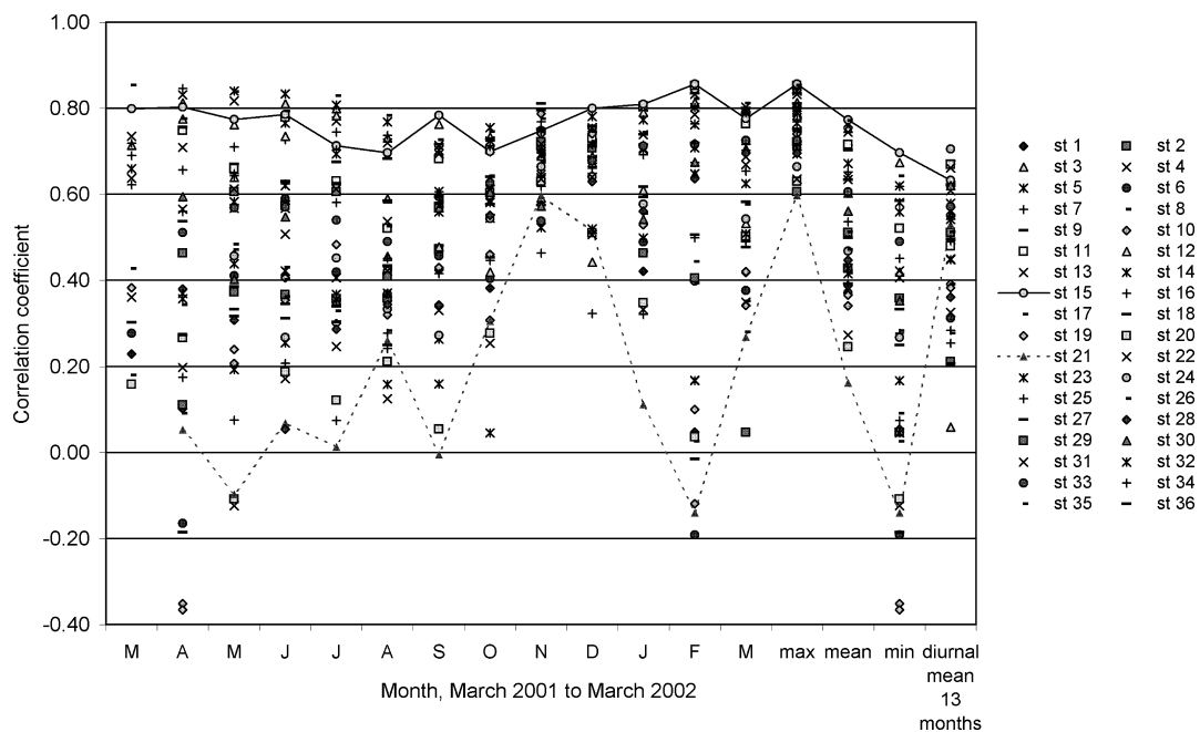
Fig. 4. Correlation coefficients between the hourly measured and modelled concentrations. Max, mean and min refer to the highest, average and lowest monthly correlation coefficients, respectively.
