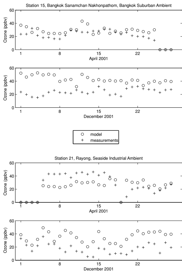
Fig. 5. Diurnal mean of measured and modelled ozone at two different stations, one suburban, in Bangkok, and one seaside industrial, in Rayon, during eight weeks.
