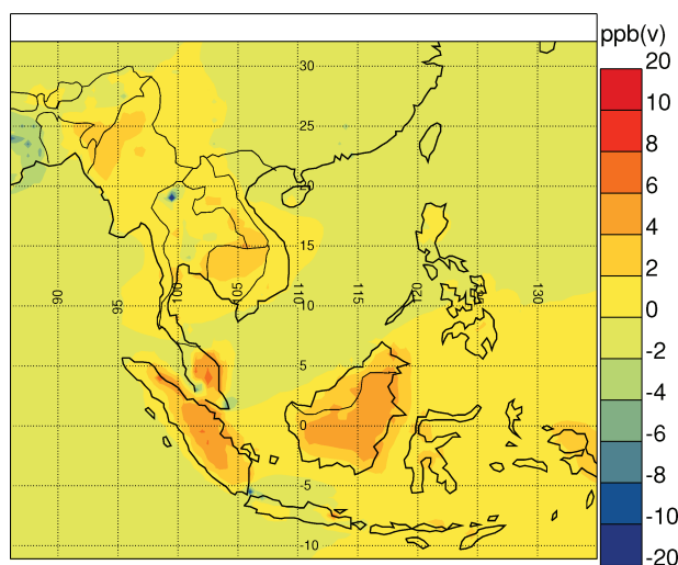
Fig. 7. Difference in annual mean ozone concentration from model set-up with 1/3 of isoprene emissions and model set-up with 100% isoprene emissions.
