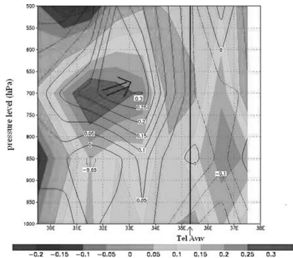
Fig. 5. The 32.5°N longitude cross-section of vertical profile (y-axis is pressure level in hPa) for the correlation between 700 hPa model temperature error \Delta T (K) at Tel Aviv (32.64°N, 35.28°E) and aerosol optical thickness (AOT) over the Eastern Mediterranean MODIS Terra gridpoints (see Section 2.1). The value of \Delta T is equal to (MM5 analysis 12 UTC) – (MM5 + forecast hours). Correlation for April 2001, 2002, 2004 & 2005 is for noon observations (12 UTC). Shaded areas are for \Delta T (+24) and black contour lines are for \Delta T (+12). The vertical bold line at longitude 35.28°E corresponds to the Tel Aviv model gridpoint.
