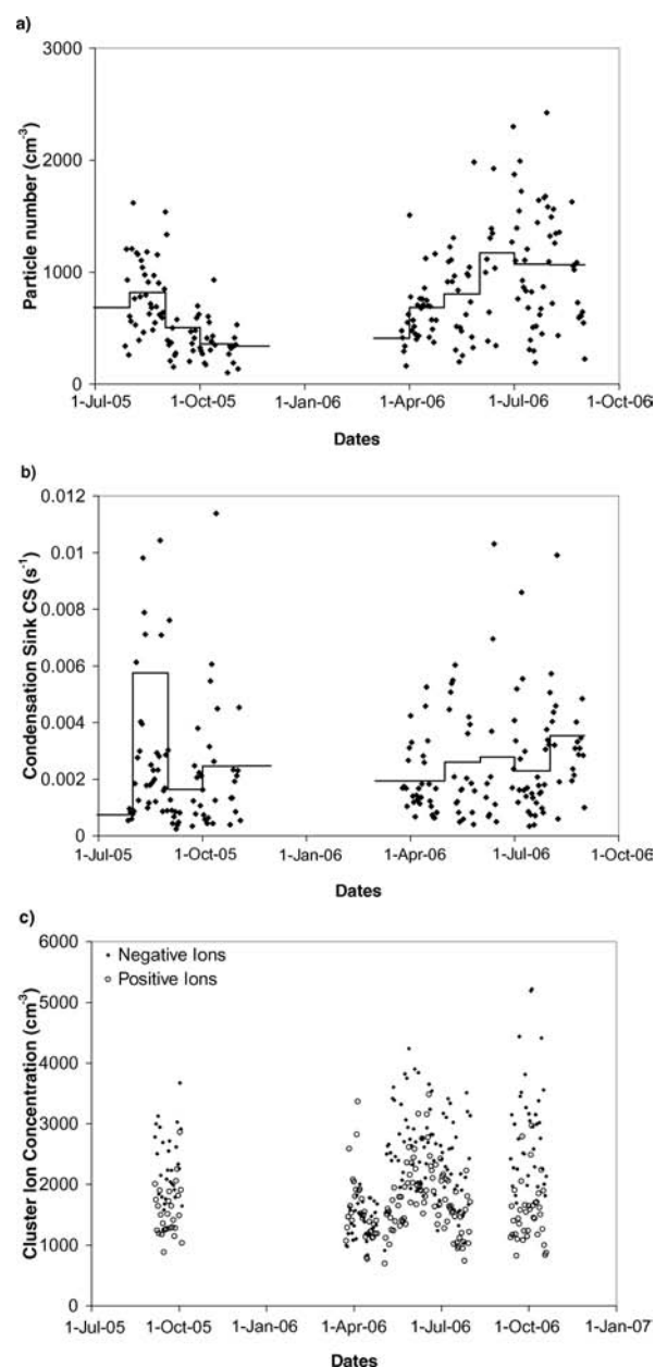
Fig. 2. Daily and monthly averages of (a) number concentration of particles in the size range 10–500 nm in diameter and (b) condensation sink (CS) estimated from the aerosol particle size distributions (SMPS data). (c) Daily averages of negative and positive cluster ions according to the fit of a lognormal distribution with a modal diameter smaller than 1.3 nm to the size distributions of the naturally charged particles in the diameter range 0.4–40 nm (AIS data). The grand average for the negative and positive cluster ion concentrations are 2380 and 1650 \text{ cm}^{-3} , respectively.
