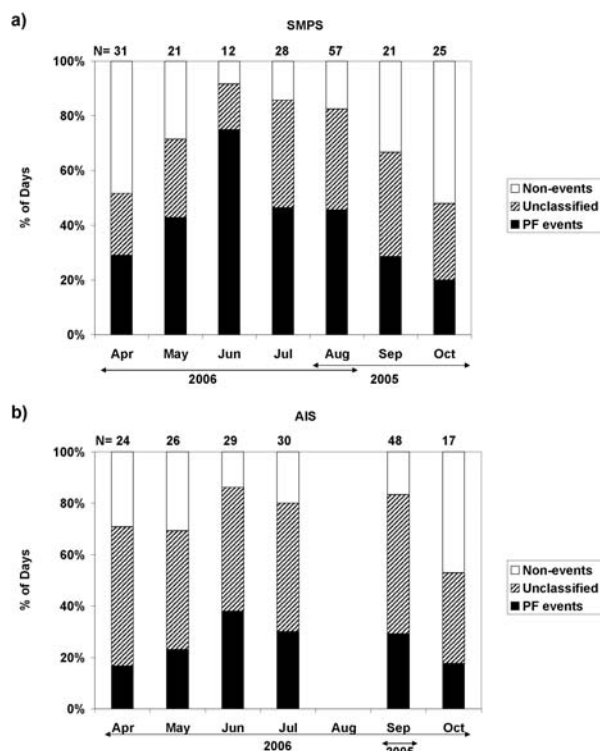
Fig. 5. Seasonality of days with particle formation events from (a) the SMPS and (b) the AIS. N represents the number of days with valuable data during each month. Black bars, particle formation event days; white bars, non-event days and striped bars, unclassified days.
