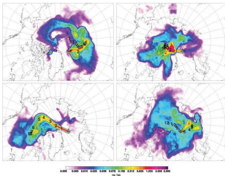
Fig. 1. Representative FLEXPART images, exemplifying the major differences in pathways and source regions between the sampling dates. Upper left picture represents filters A4–A7 (22–23 May). Upper right-hand side picture represents filters C1, E4–E6 (27 May, 3 June). Lower left-hand side picture represents filters G1, G4, H4, H5 (7, 8 and 11 June). Lower right-hand side picture represents filter J1 (14 June) (Warmer colour—higher contribution; numbers stand for days past until arrival).
