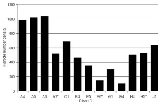
Fig. 4. Average number density ( \text{cm}^{-3} ) of particles larger than 100 nm diameter for the time intervals corresponding to the analysed filters. Filter id with '*' indicate that a major part of the time the sampling was in cloudy conditions.
