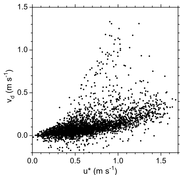
Fig. 4. Scatter plot of the fogwater deposition velocities v_d versus friction velocity u^* . All 30 min averages are shown. A 'negative deposition velocity' corresponds to a net emission flux.
