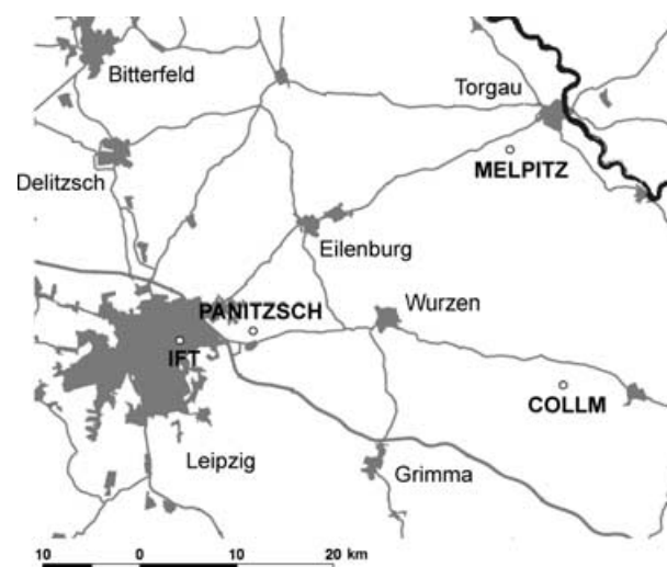
Fig. 1. Map of the measurement site during SATURN showing the location of the measurement sites Melpitz, Collm, Panitzsch and IFT.
