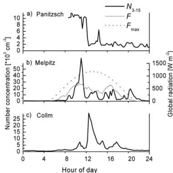
Fig. 8. Evolution of number concentration N_{3-15} in the size range of 3–15 nm for the stations Panitzsch, Melpitz and Collm and global radiation F and maximum global radiation F_{\max} in Melpitz on 11 June 2002.
