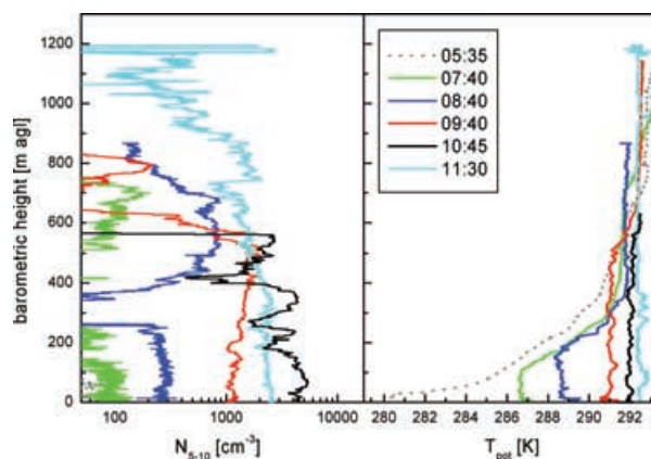
Fig. 5. Selected vertical profiles of N_{5-10} in the size range of 5–10 nm (left-hand side) and potential Temperature T_{\text{pot}} (right-hand side) measured on 3 June in Melpitz. Times are in CEST and valid for the mean of profile.
