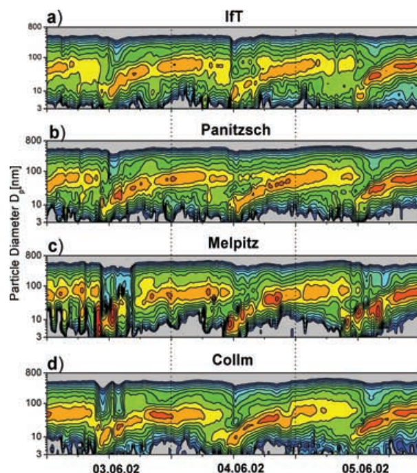
Fig. 2. Evolution of normalized number size distributions from 3 June (00:00 CEST) to 5 June (24:00 CEST), 2002 at the stations IfT, Panitzsch, Melpitz, and Collm. The colours represent particle number concentration divided by the total number concentration, grey represents relatively low concentrations and red means high concentrations.
