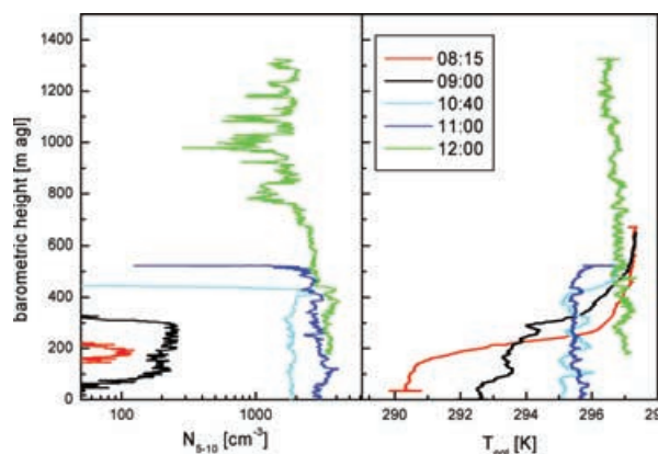
Fig. 6. Selected vertical profiles of N_{5-10} in the size range of 5–10 nm (left-hand side) and potential Temperature T_{\text{pot}} (right-hand side) measured on 4 June in Melpitz. Times are in CEST and valid for the mean of profile.
