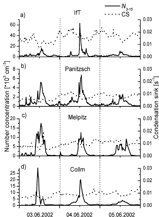
Fig. 3. Evolution of the number concentration N_{3-15} in the size range of 3–15 nm and condensation sink CS between 3 June (0:00 CEST) and 5 June (24:00 CEST), 2002 at the stations IfT, Panitzsch, Melpitz and Collm.
