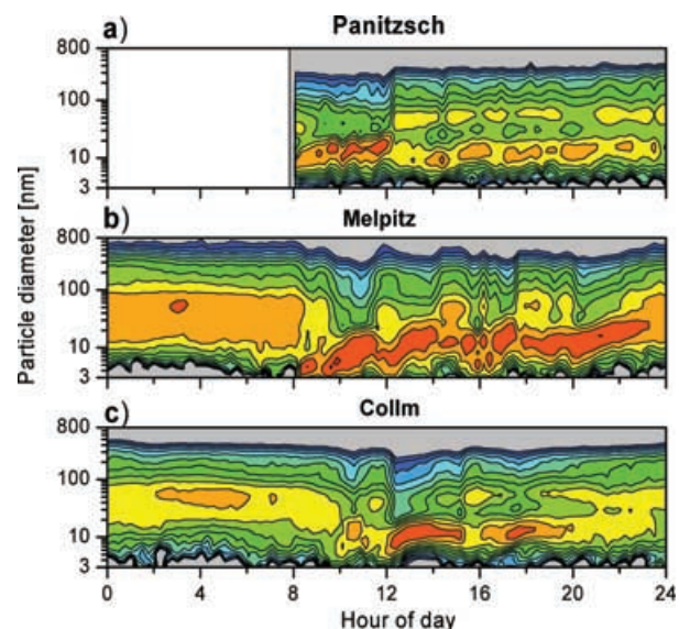
Fig. 7. Evolution of normalized number size distributions on 11 June 2002 at the stations Panitzsch, Melpitz and Collm; grey represents relatively low concentrations and red means high concentrations.
