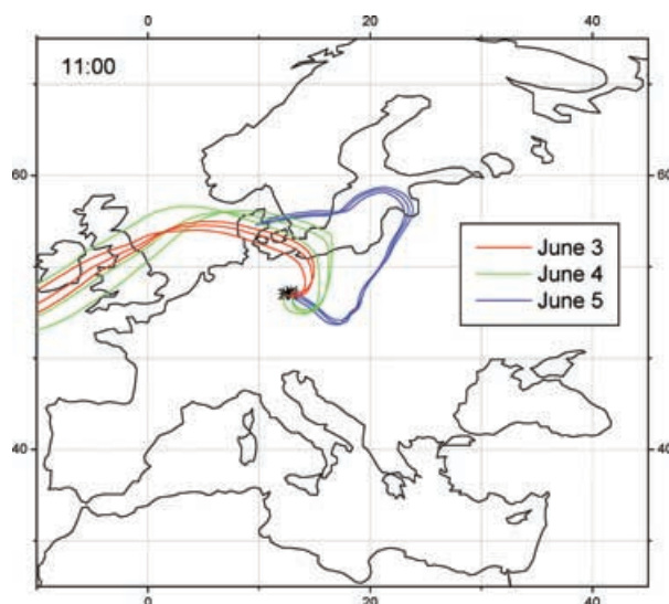
Fig. 4. 144 hr back-trajectories (HYSPLIT) for the stations Melpitz, Collm and IfT on 3, 4 and 5 June arriving at 11:00 CEST in a height of 100 m asl.
