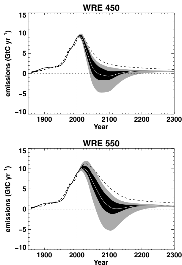
Fig. 2. Observationally constrained permissible emissions for WRE450 and WRE550 scenarios. Only parameter combinations which are consistent with historical emissions are chosen. The central white line represents the simple model results when run with the best fit parameters to HadCM3LC. The central black shading shows the uncertainty range for a climate sensitivity of 3 K (as fitted to HadCM3LC). The grey shading shows the range for climate sensitivity in the IPCC-TAR range of 1.5–4.5 K. The dashed lines show the emissions profiles from Wigley et al. (1996).
