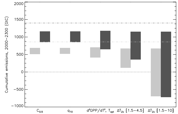
Fig. 1. Uncertainty in cumulative permissible emissions from 2000 to 2300 due to uncertainty in the carbon cycle sensitivity to \text{CO}_2 or climate, and climate sensitivity. The bars show the range of cumulative emissions when each parameter is varied individually within the range stated in the text. Results are shown for climate sensitivity values from 1.5 to 4.5 K, and from 1.5 to 10 K. Pale bars show results for stabilization at 450 ppm following the WRE450 \text{CO}_2 scenario, and dark bars likewise for WRE550. The dashed lines represent the level of cumulative emissions from Wigley et al. (1996).
