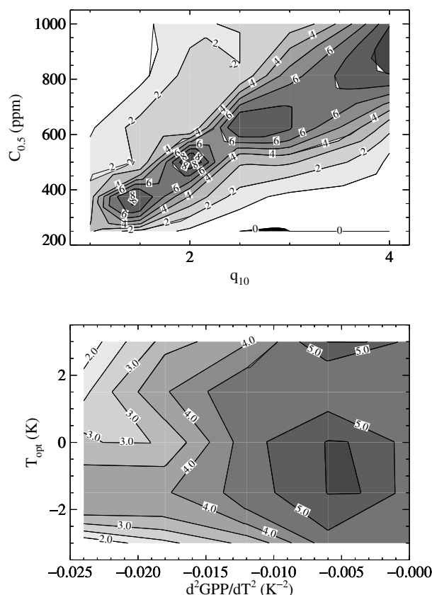
Fig. 5. Joint frequency distribution of (a) q_{10} and C_{0.5} as constrained by the historical emissions record and (b) same for d^2GPP/dT^2 and T_{opt} . The contours show the percentage frequency of occurrence of combinations of parameter values within the set of 127 simulations which match the historical record of emissions.
