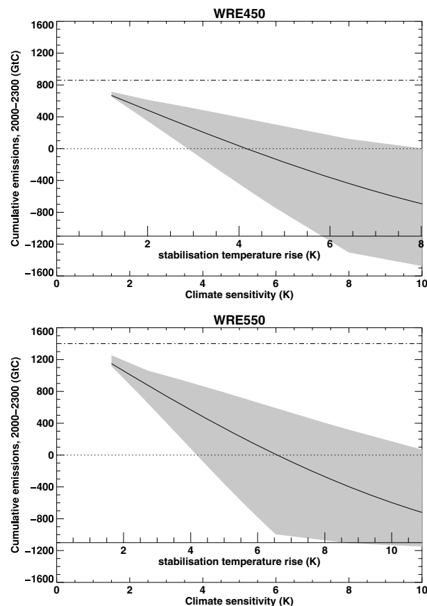
Fig. 3. Sensitivity of cumulative permissible \text{CO}_2 emissions from 2000 to 2300 to variations in the climate sensitivity. Results are shown for stabilization following WRE450 (top panel) and WRE550 (bottom panel) scenario. The solid lines show a strong decrease in cumulative emissions for increasing climate sensitivity when carbon cycle feedbacks are considered. Dot-dashed lines show values from Wigley et al. (1996) when these feedbacks are neglected. The shaded regions show the range of uncertainty when the carbon cycle parameters are varied, but constrained by the historical emissions. For reference, the global temperature change by 2300 is marked on a separate axis.
