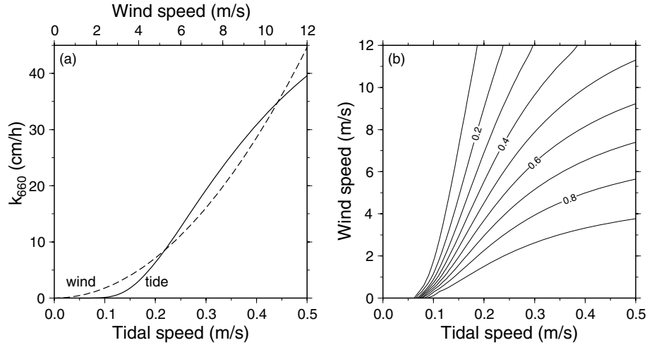
Fig. 4. (a) Dependency of the gas transfer velocities on the wind and tide and (b) the ratio of the gas transfer velocities due to the tide to the sum of the velocities due to the tide and wind ( k_t/[k_t + k_w] ). k_{660} is the gas transfer velocity for a Schmidt number of 660, the value for \text{CO}_2 in seawater at 20^\circ\text{C} .
