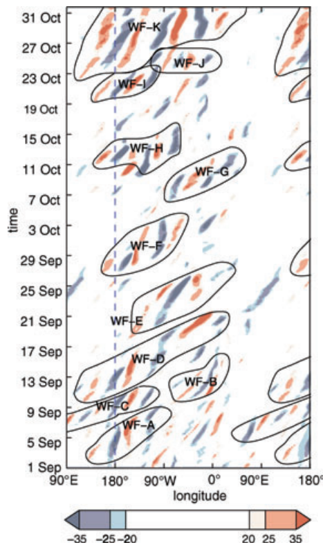
Fig. 3. Weighting function Hovmöller diagram of the meridional wind \hat{v} ( \text{ms}^{-1} , colour shaded) at \Theta = 330 K for September and October 2008. Visually identified RWT are surrounded by a black line and labelled WF-A to WF-K.
