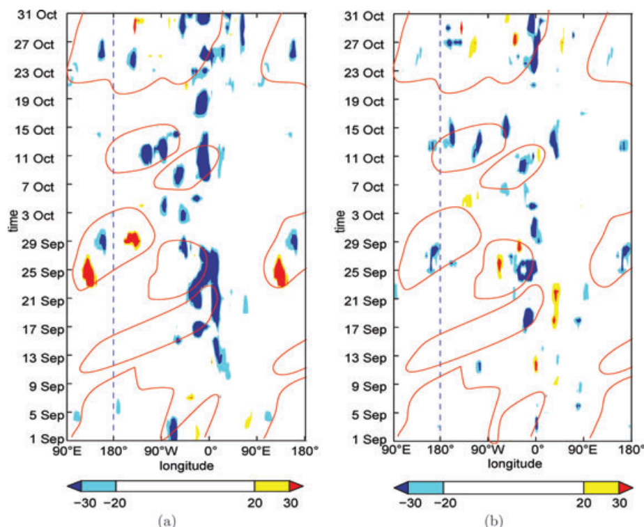
Fig. 11. Hovmöller diagrams of the wave breaking index for September and October 2008. (a) P1 ( \text{m}^2 \text{s}^{-2} , positive values) and P2 ( \text{m}^2 \text{s}^{-2} , negative values). (b) LC1 ( \text{m}^2 \text{s}^{-2} , negative values) and LC2 ( \text{m}^2 \text{s}^{-2} , positive values).
