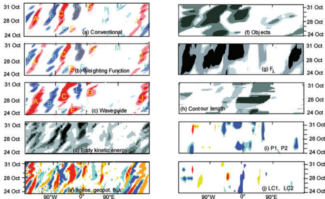
Fig. 13. Period of October 24 to 31 for the Hovmöller diagrams as described in Section 3.
