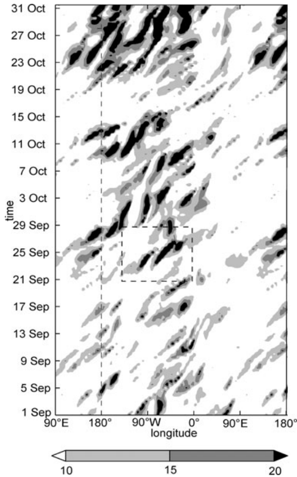
Fig. 5. Hovmöller diagram of \overline{K_e} (in 10^5 \text{ J m}^{-2} ) for the episode September and October 2008. The data are vertically integrated between 1000 and 100 hPa and averaged over a latitude belt between 40^\circ and 60^\circ \text{N} . The temporal resolution of the data for this analysis is 12 h. The dashed box refers to the area of Fig. 8.
