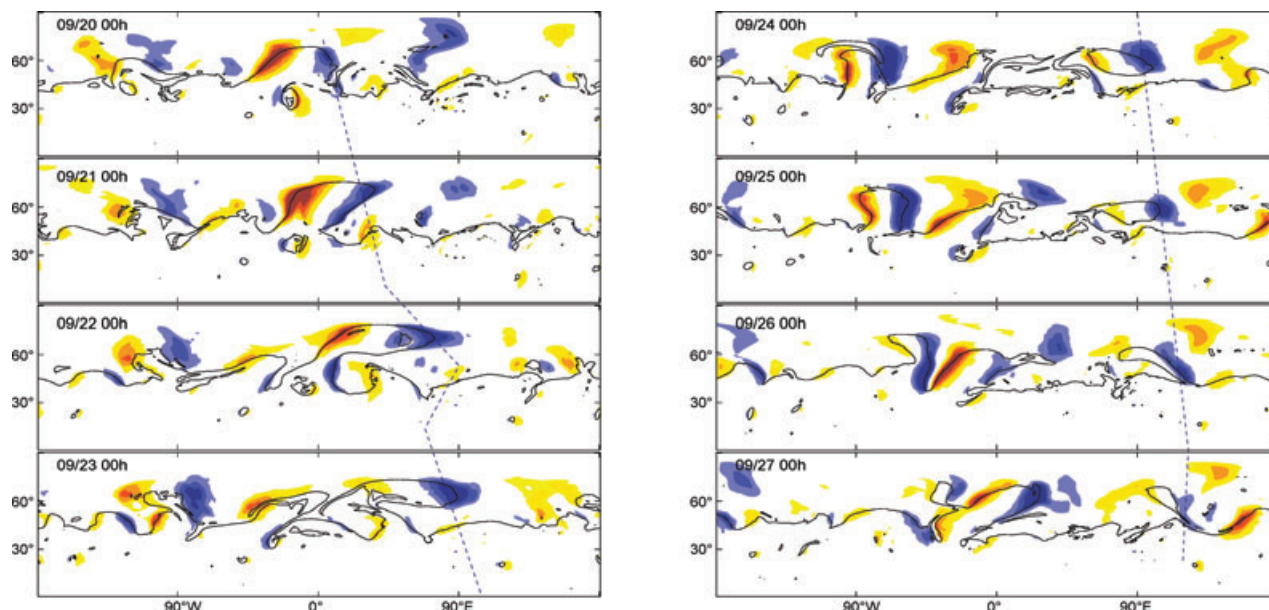
Fig. 14. Representation of the synoptic situation during the short episode from September 20 to 27 on the 330 K isentropic surface. Black line: 2 PVU-contour, bluish colours: negative meridional wind [ (-20, -30, -40, -50) \text{ m}^2 \text{ s}^{-2} ], reddish colours: positive meridional wind [ (20, 30, 40, 50) \text{ m}^2 \text{ s}^{-2} ]. The blue dashed line denotes the position of the trough discussed in the text.
