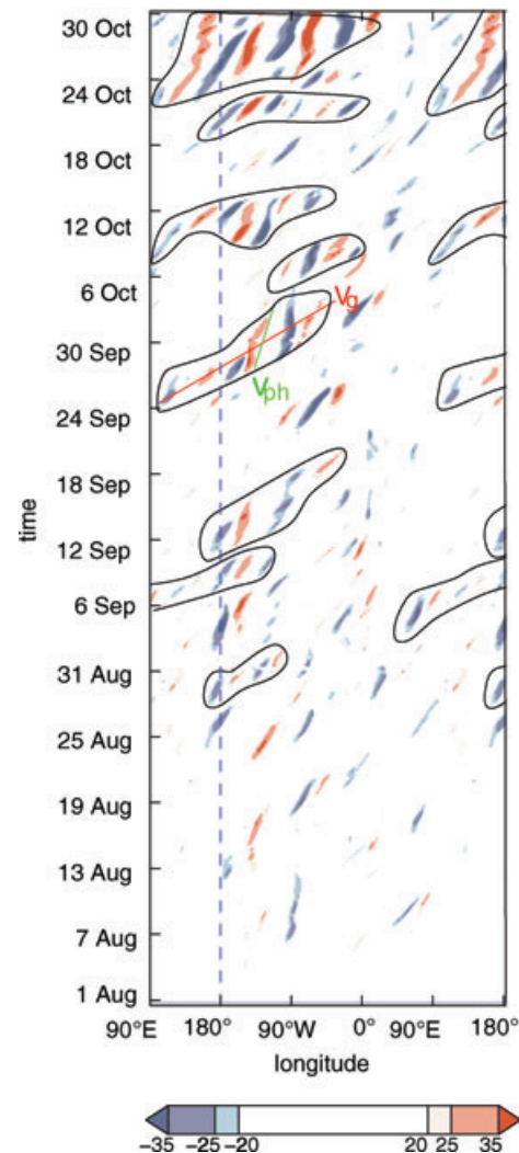
Fig. 1. Conventional Hovmöller diagram of the meridional wind v ( \text{m s}^{-1} ; colour shaded) on the 330 K isentropic surface, averaged between 40^\circ and 60^\circ\text{N} for August through October 2008. For ease of viewing the region west of the date line was plotted twice in a wrap-around manner. Visually identified RWT are surrounded by a black line. The red and green line illustrate how the group and phase velocity can be obtained from this type of diagram.
