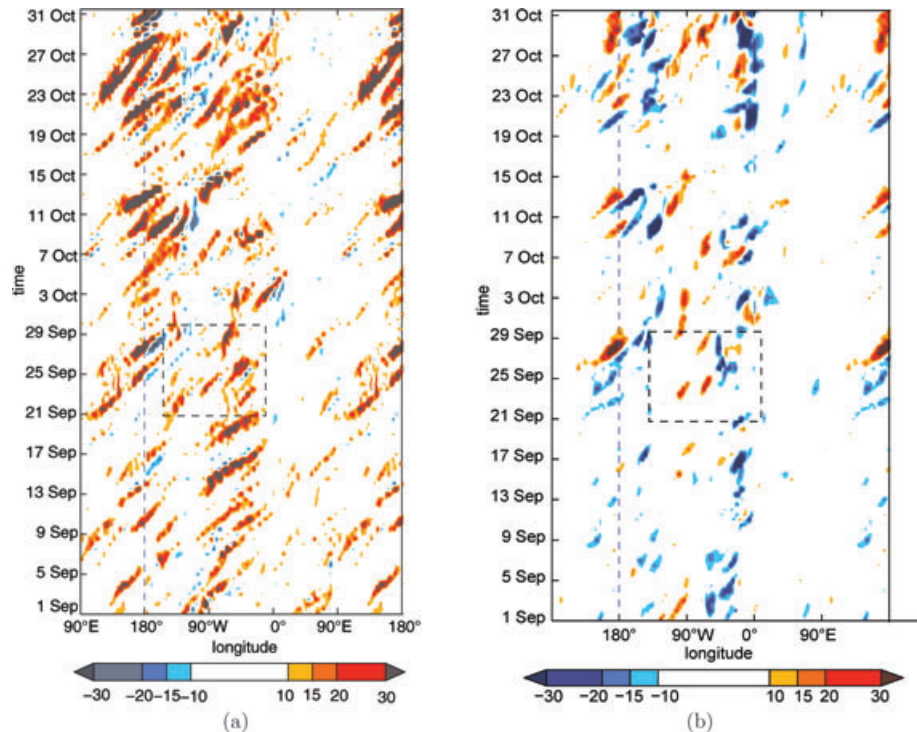
Fig. 6. Hovmöller diagrams for September and October 2008 of the generation of the eddy kinetic energy. (a) Term A ( \text{Wm}^{-2} ) and (b) term B ( \text{Wm}^{-2} ). All quantities are vertically integrated between 1000 to 100 hPa and averaged over a latitude belt between 40^\circ and 60^\circ N. The temporal resolution of the data for this analysis is 12 h. The dashed box refers to the area of Fig. 8.
