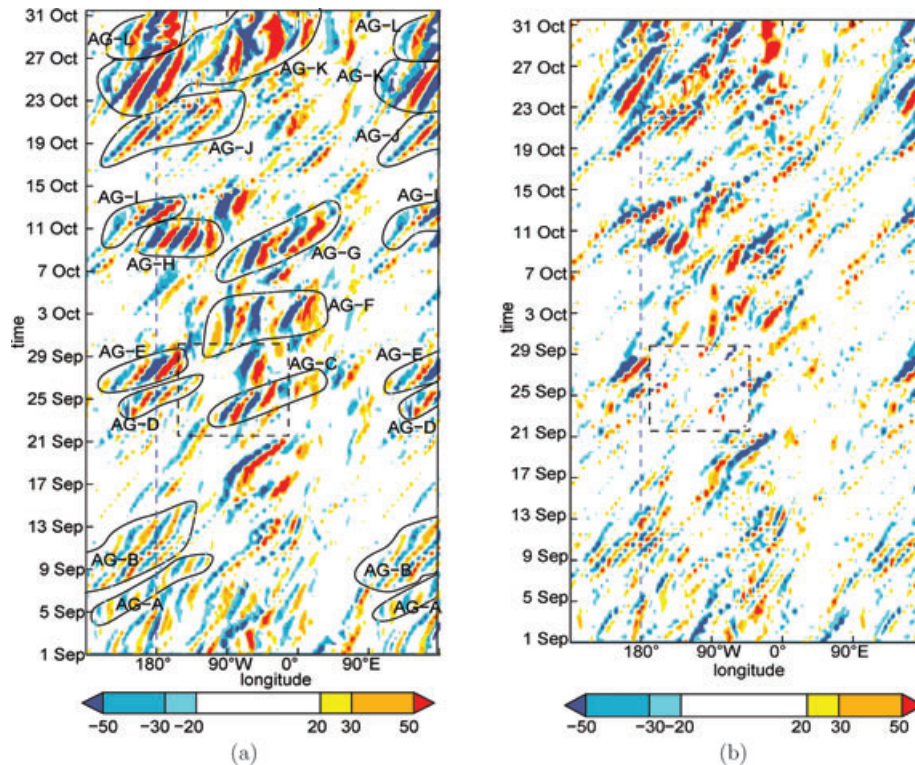
Fig. 7. Hovmöller diagram for September and October 2008 of the convergence of eddy kinetic energy. (a) Term C (divergence of the ageostrophic geopotential flux) ( \text{Wm}^{-2} ) and (b) term D ( \text{Wm}^{-2} ). All quantities are vertically integrated between 1000 to 100 hPa and averaged over a latitude belt between 40^\circ and 60^\circ N. The temporal resolution of the data for this analysis is 12 h. The dashed box refers to the area of Fig. 8.
