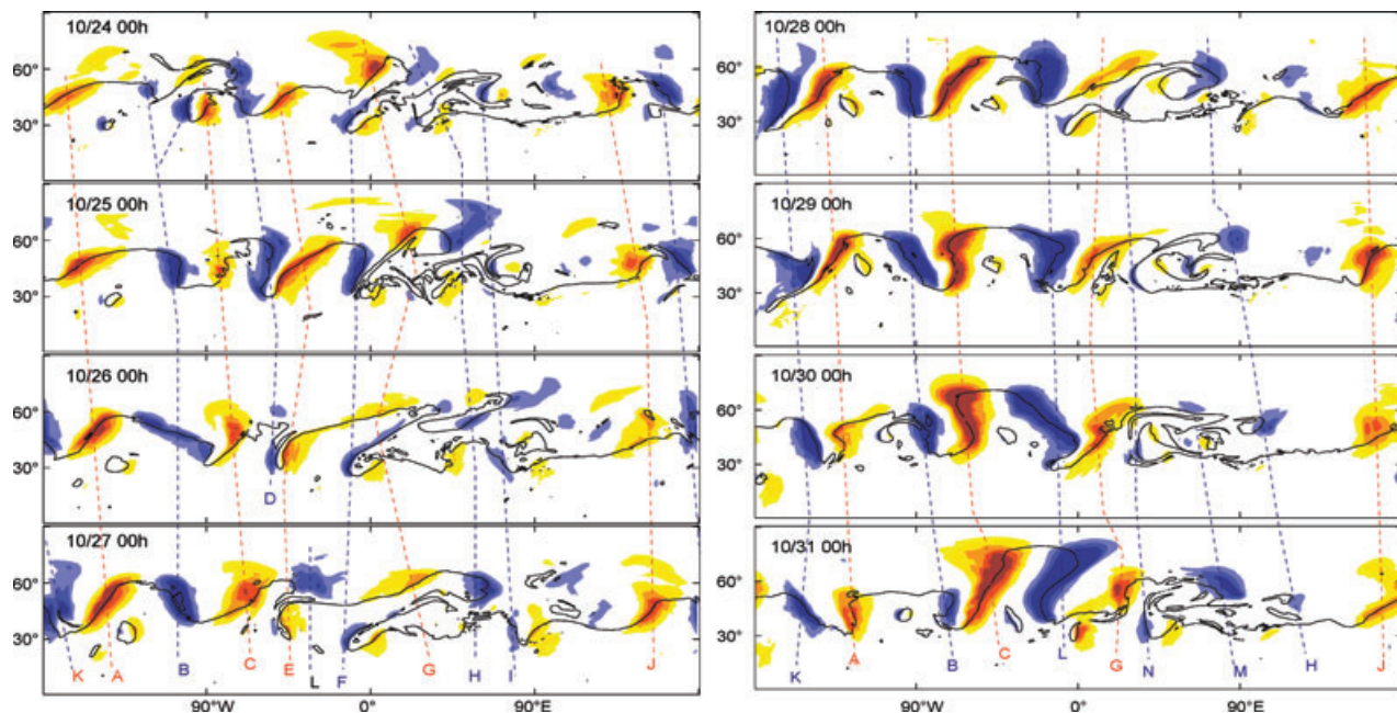
Fig. 12. Representation of the synoptic situation during the short episode from October 24 to 31 on the 330K isentropic surface. Black line: 2 PVU-contour, bluish colours: negative meridional wind [(-20, -30, -40, -50) \text{ m}^2 \text{ s}^{-2}] , reddish colours: positive meridional wind [(20, 30, 40, 50) \text{ m}^2 \text{ s}^{-2}] . The blue (negative meridional wind) and red (positive meridional wind) dashed lines denote the position of the extrema in the meridional wind, that are also indicated with the same labels in Fig. 13.
