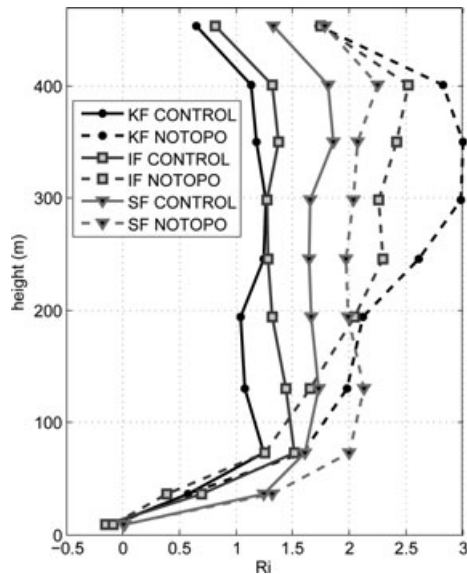
Fig. 9. The mean Richardson number ( Ri ) profiles over Storfjorden (SF), Isfjorden (IF) and Kongsfjorden (KF) in the CONTROL and NOTOPO simulations.
