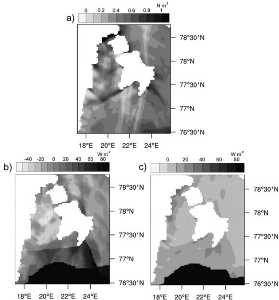
Fig. 5. Turbulent surface fluxes of (a) momentum \tau , (b) sensible heat H and (c) latent heat LE in Storfjorden for a northeasterly flow on 13 February 2008 at 12 UTC. The land area is masked out.
