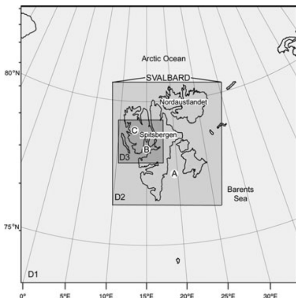
Fig. 1. Domains D1, D2 and D3, used in WRF model, with resolutions of 9, 3 and 1 km, respectively. The studied fjords are: (A) Storffjorden, (B) Isfjorden and (C) Kongsfjorden.
