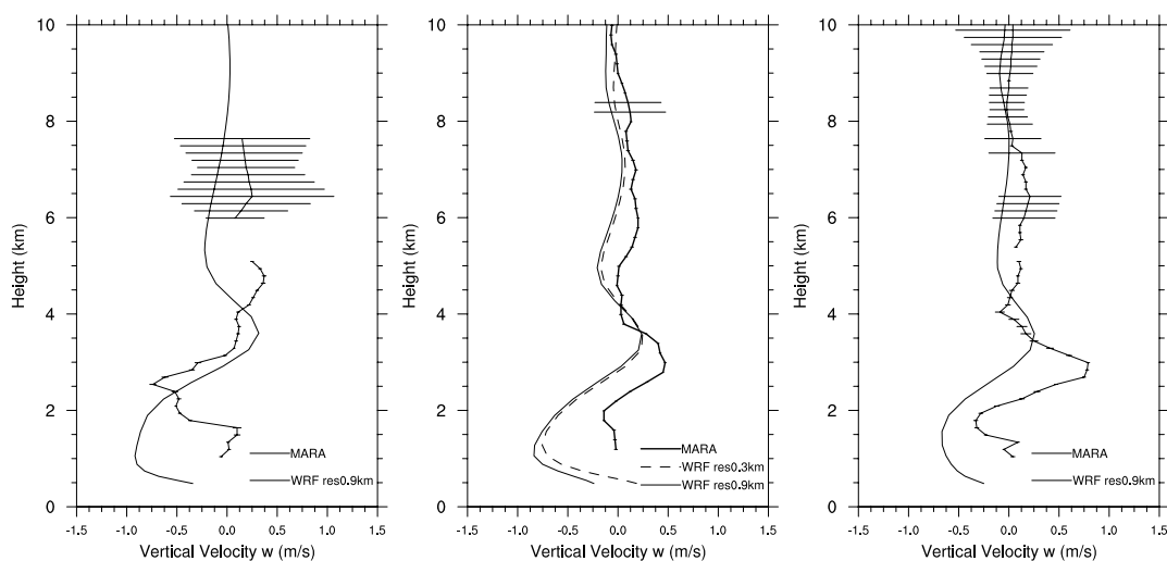
Fig. 9. Profiles of vertical wind velocity at Basen nunatak at 2007-12-10 06 UTC (left-hand panel), 2007-12-31 00 UTC (middle panel) and 2008-01-12 12 UTC (right-hand panel) from WRF simulations and MARA measurements.
