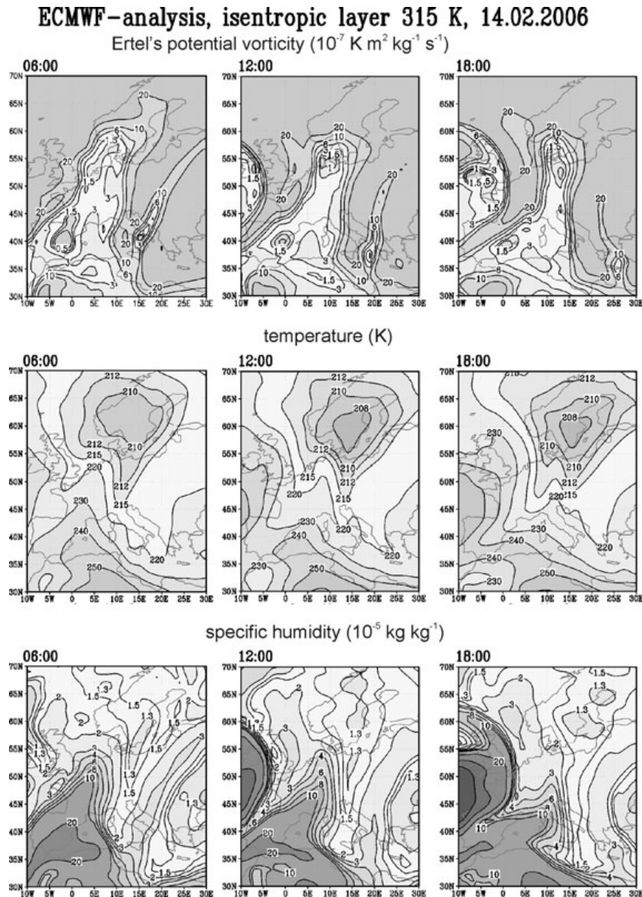
Fig. 4. Regional maps of EPV, temperature and specific humidity at the 315 K isentropic surface on 14 February 2006 for 6:00, 12:00 and 18:00 UT.
