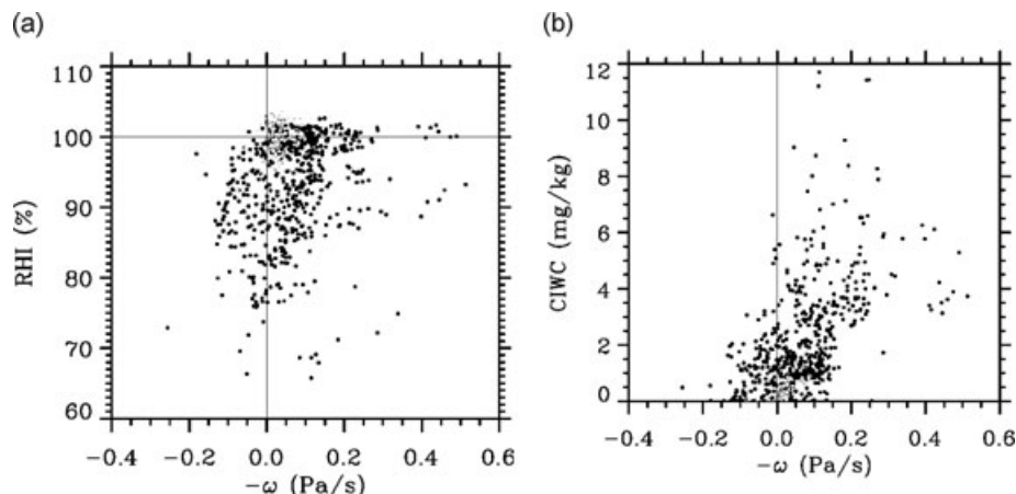
Fig. 8. Scatter plot between (a) vertical velocity (Pa/s) and RH (%); and (b) vertical velocity (Pa/s) and updraft and CIWC (mg/kg) along the backward trajectories released in a box centred over Kühlungsborn at 240 hPa on 14 February 2006, 12:00UT. The trajectory is every hour (more details see text in Section 3.5).
