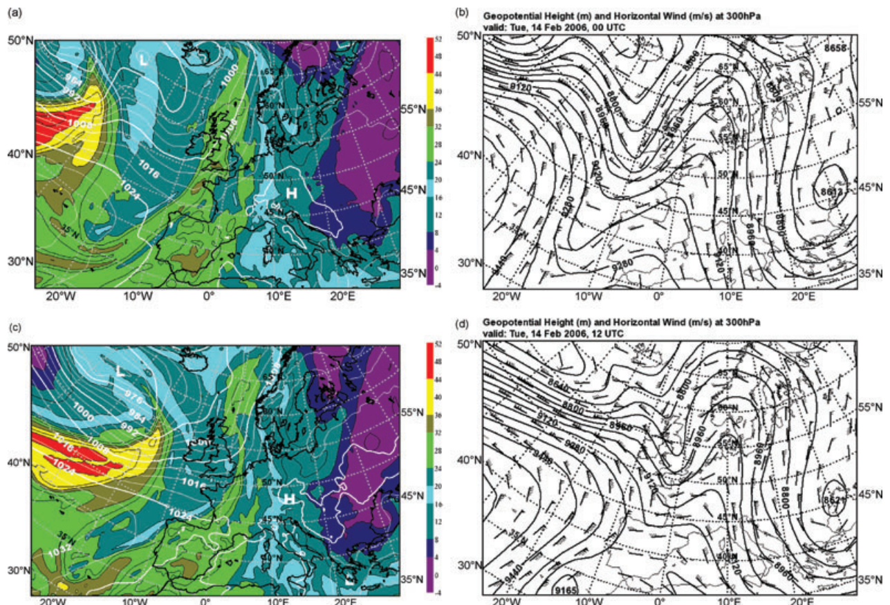
Fig. 1. Operational T799/L90 analyses of the ECMWF on 14 February 2006 valid at (a), (b) 0:00 UT and (c), (d) 12:00 UT, respectively. Panels (a) and (c) show the mean sea level pressure (hPa, white solid lines) and equivalent potential temperature (°C, color bar) at the 850 hPa level, and panels (b) and (d) depict the geopotential height (m, solid lines) and horizontal winds (m/s, barbs) at the 300 hPa pressure level.
