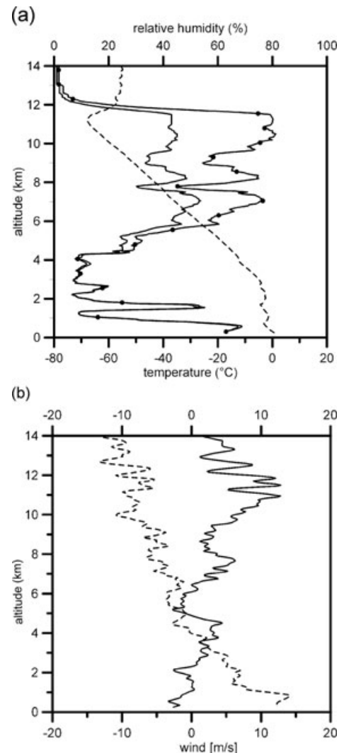
Fig. 6. Vertical profiles of (a) temperature ( ^{\circ}\text{C} ; dashed line), \text{RHw} (%; thin line) and \text{RHi} (%; line with dots). (b) Zonal (full) and meridional (dashed) winds ( \text{m s}^{-1} ) observed by a radiosonde launched at Kühlungsborn on 14 February 2006, 14:26 UT.
