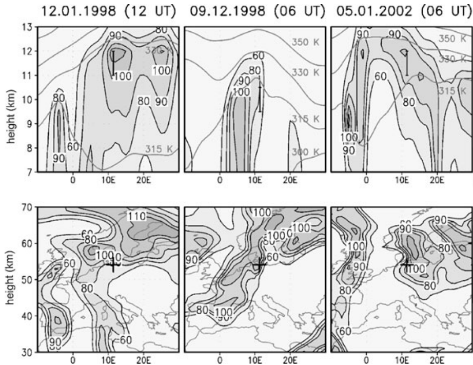
Fig. 10. Maps of ECMWF analysis for RH_i > 60\% on 12 January 1998, 12:00 UT, on 9 December 1998, 6:00 UT and on 5 January 2002, 6:00 UT are shown. Upper panel: Height-longitude crosssection at 54^\circ N with different isentropic layers (lines). The bar marks the altitudinal region where the lidar at Kühlungsborn detected cirrus clouds. Lower panel: Latitude-longitude crosssection at 330 K (left) and 315 K (middle, right) isentropic layer, respectively. A cross marks the location of Kühlungsborn.
