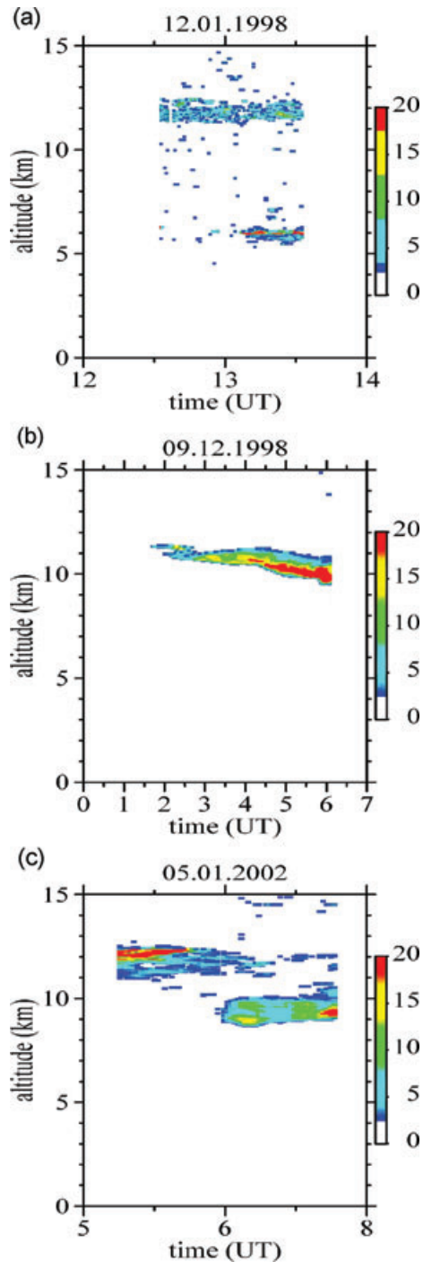
Fig. 9. Aerosol backscatter ratio R_\lambda at 532 nm wavelength above Kühlungsborn; (a) on 12 January 1998, (b) on 9 December 1998 and (c) on 5 January 2002.
