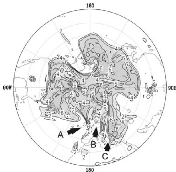
Fig. 3. EPV map of ECMWF analysis at the 315 K isentropic surface on 14 February 2006, 12 UT. Contour interval is 2 PVU ( 1 \text{ PVU} = 10^{-6} \text{ K m}^2 \text{ kg}^{-1} \text{ s}^{-1} ). Values larger than 2 PVU are shaded. Arrows A, B, and C mark special anticyclonic air masses which are described in Section 3.3.
