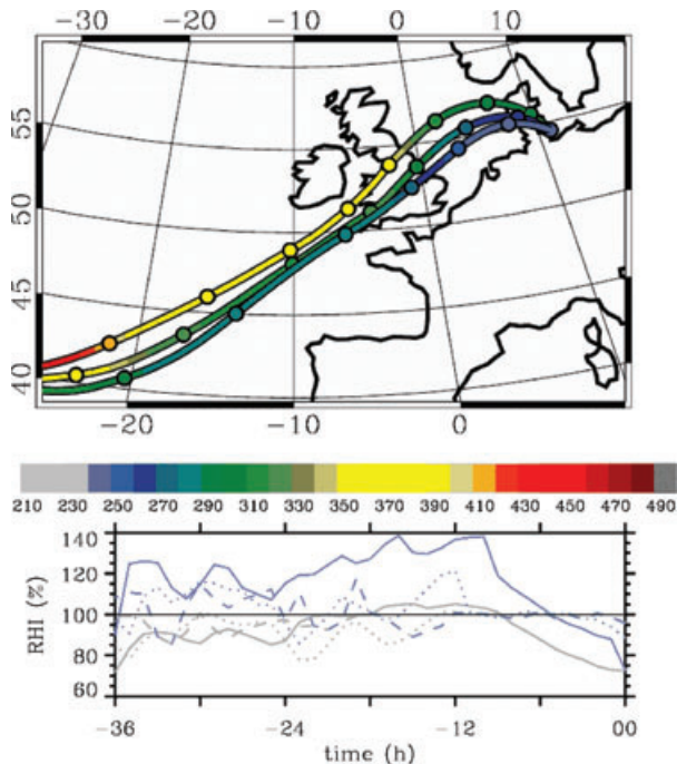
Fig. 7. Upper panel: Positions and pressure (hPa, color coded) of the center of gravity of trajectories launched inside the box ( 54^{\circ} N, 55^{\circ} N) and ( 10^{\circ} E, 12^{\circ} E) at 300, 260, and 240 hPa, respectively. Circles denote 12 hour increments. Lower panel: RH along the mean trajectories released at 300 (solid lines), 260 (dotted), and 240 hPa (dashed), respectively. The grey lines denote RH averaged over all trajectories, whereas the blue lines denote RH calculated with the specific humidity averaged over all trajectories added by its rms deviation.
