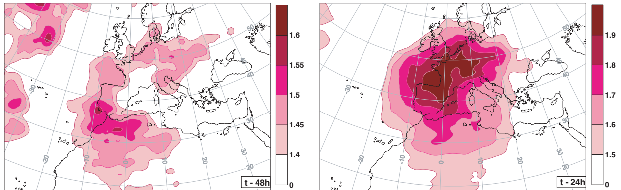
Fig. 9. Mean sensitivity field for all 25 cyclone types computed over all considered precursor conditions and levels (mb, shaded) for t = 48 h (left-hand panel) and t = 24 h (right-hand panel). Note the scale change between figures.
