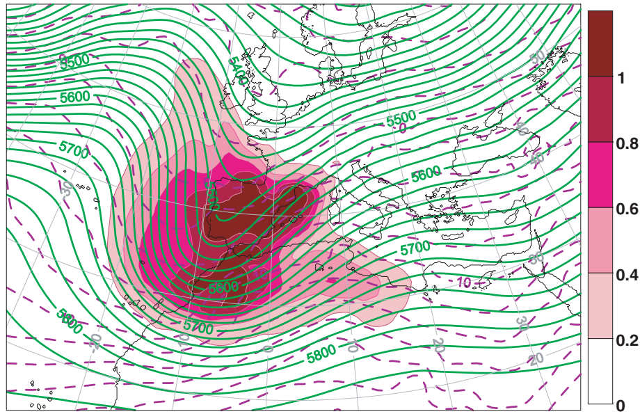
Fig. 8. Vertically averaged adjoint-computed sensitivity fields (darker shaded colours show larger sensitivities) for cluster 5 at t = 48 h. Geopotential height field at 500 hPa (gpm, solid lines) and temperature field at 850 hPa ( ^{\circ}\text{C} , dashed lines) averaged over all cluster's members (adapted from Jansà and Homar, 2006).
