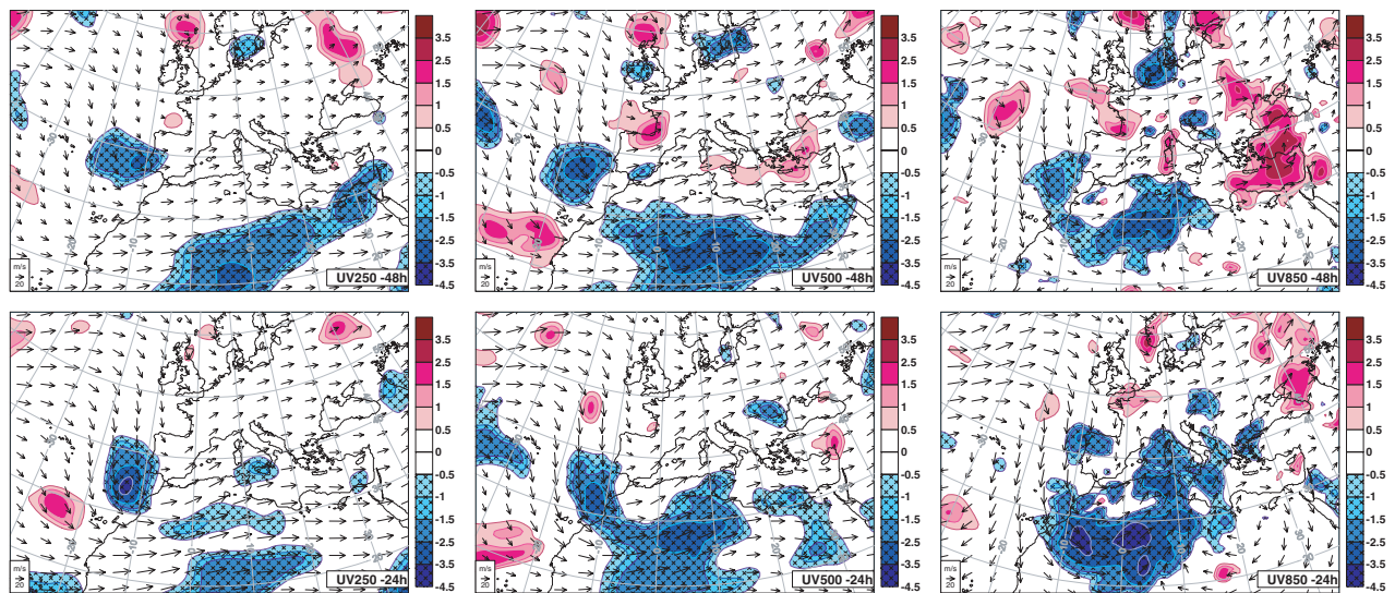
Fig. 5. Sensitivity of the response function (mb, shaded) with respect to wind speed (cluster's mean field: \text{ms}^{-1} , vectorial field) at t - 48 h (upper panels) and t - 24 h (lower panels) for cluster 5.
