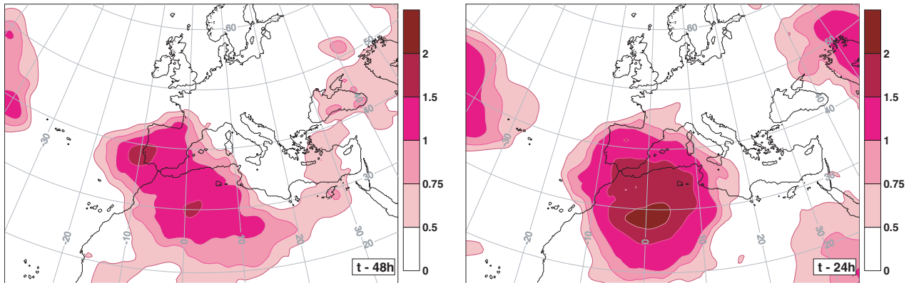
Fig. 6. Mean sensitivity field over all considered precursor conditions fields and levels (mb, shaded) for t - 48 h (left-hand panel) and t - 24 h (right-hand panel) for cluster 5.
