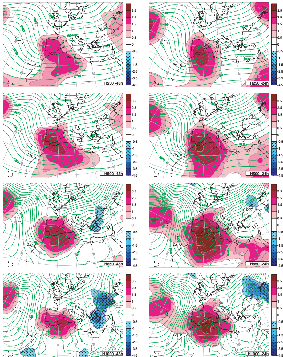
Fig. 3. Sensitivity of the response function (mb, shaded) with respect to geopotential height (cluster's mean field: gpm, solid lines) at t - 48 h (left-hand side column) and t - 24 h (right-hand column) for cluster 5.
