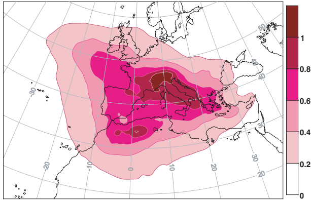
Fig. 10. Mean adjoint sensitivity field to central cyclone pressure at t - 48 h weighted by the intense cyclone frequency within the database (darker colours indicate higher sensitivities; adapted from Jansà and Homar, 2006).
