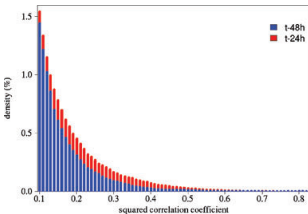
Fig. 7. Distribution of squared correlation coefficients corresponding to all S_{ij} considered in this study for t - 48 and t - 24 h.
