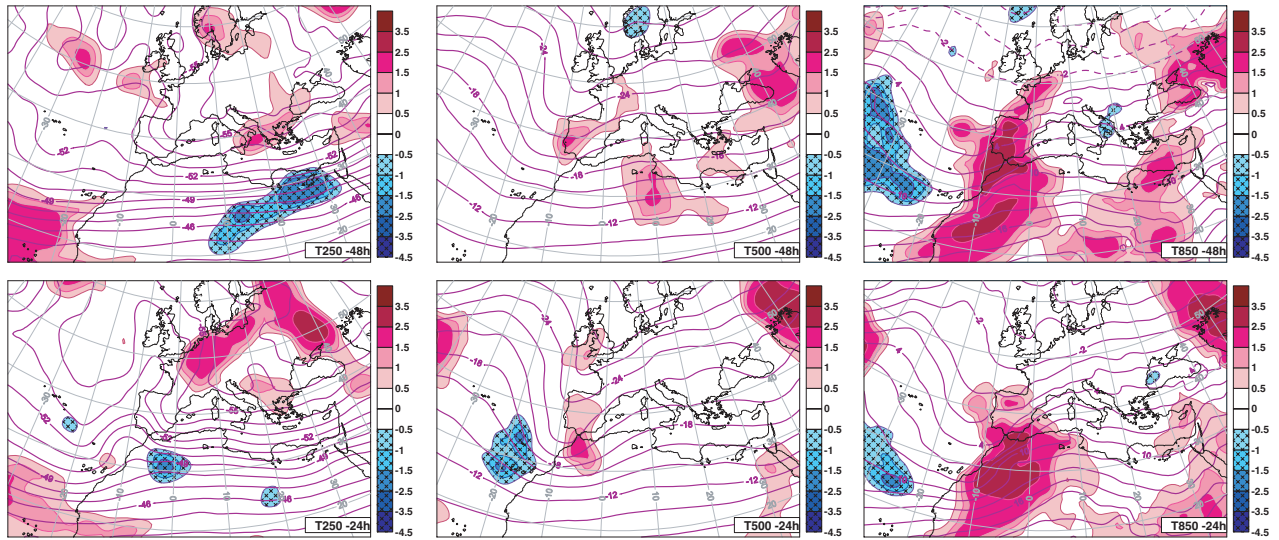
Fig. 4. Sensitivity of the response function (mb, shaded) with respect to temperature (cluster's mean field: ^{\circ}\text{C} , solid lines denote positive values and dashed lines denote negative values) at t - 48 h (upper panels) and t - 24 h (lower panels) for cluster 5.
