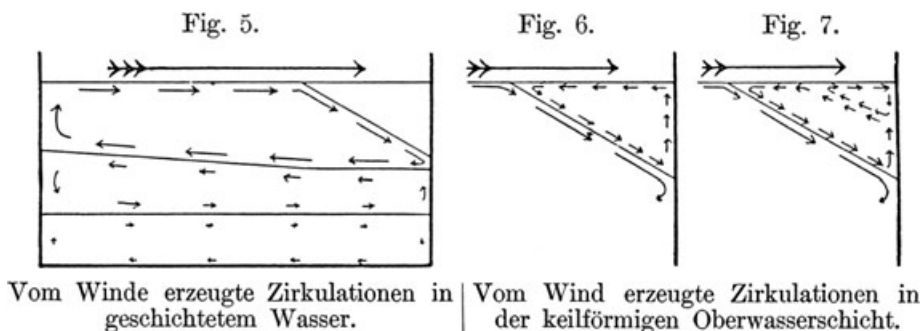
Fig. 5. Wind-driven circulations in stratified water. Figs. 6 and 7. Wind-driven circulations in the wedge-shaped surface layer.
