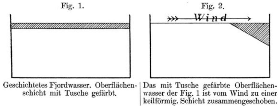
Fig. 1. Stratified fjord water. Note: Surface layer coloured with ink. Fig. 2. The ink-coloured surface water of Fig. 1 has been pushed into a wedge-shaped layer by the wind.
