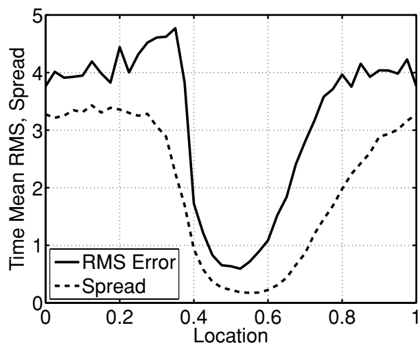
Fig. 1. Ensemble mean rms error and ensemble spread averaged over last 2000 steps of a Lorenz-96 model assimilation with a perfect model and no inflation (case P-No). Twenty observations with error variance 1.0 are equally-spaced in the region between 0.405 and 0.595 and assimilated every time step.
