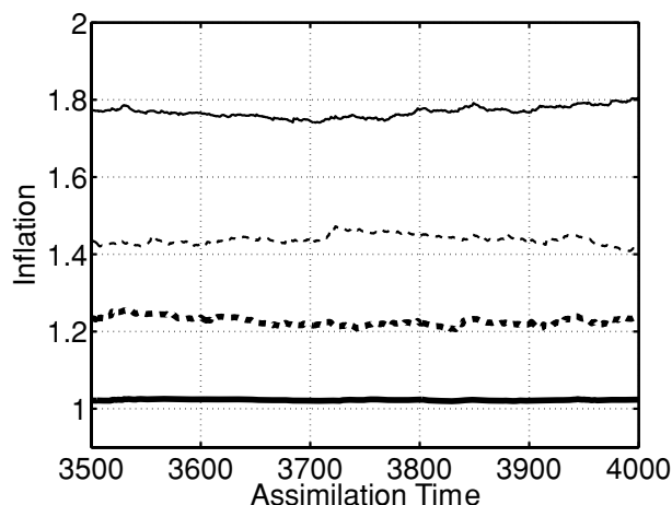
Fig. 10. Values of spatially varying inflation over last 500 assimilation times for state variables at location 0.25 (thick solid), 0.375 (thick dashed), 0.5 (thin solid) and 0.6 (thin dashed).
