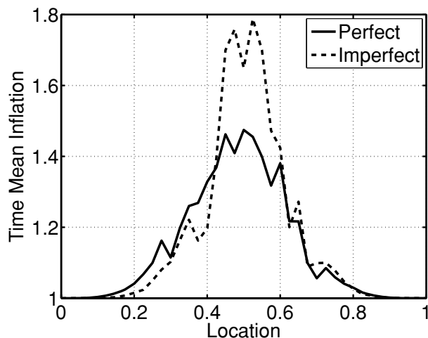
Fig. 5. Values of the adaptive inflation as a function of state variable location averaged over last 2000 time steps of perfect model (P-ST, solid) and imperfect model (I-ST, dashed) assimilations.
