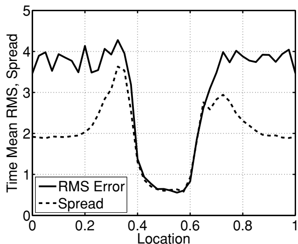
Fig. 8. As in Fig. 6 for case with an imperfect model and spatially and temporally varying adaptive inflation (case I-ST).
