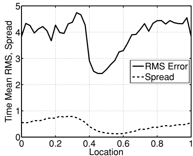
Fig. 6. Ensemble mean rms error and ensemble spread averaged over last 2000 steps of a Lorenz-96 model assimilation with an imperfect model and no inflation (case I-No). The model integration used to generate the observations had F = 8 while the assimilating model had F = 5 . Twenty observations with error variance 1.0 are equally spaced in the region between 0.405 and 0.595 and assimilated every time step.
