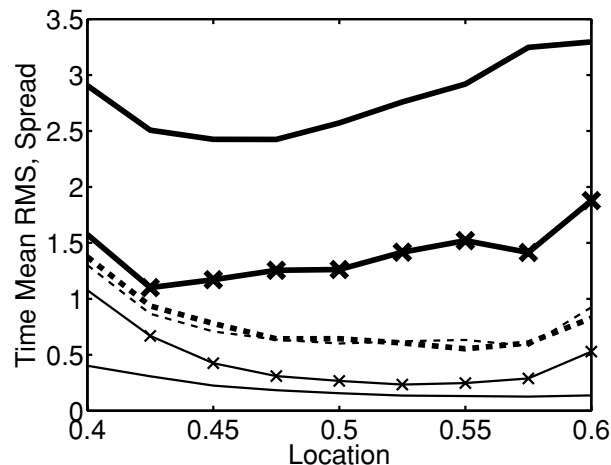
Fig. 9. rms error and spread from imperfect model cases in Figs. 6–8, displayed only over the region where observations are available. Thick lines are rms and thin lines are spread. Solid lines are no inflation case (I-No), solid with 'x' are constant inflation (I-Con) and dashed are spatially varying adaptive inflation (I-ST).
