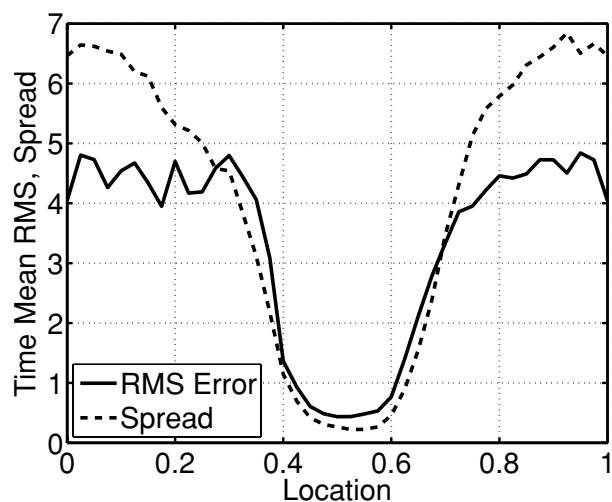
Fig. 2. As in Fig. 1 for case with a perfect model and constant 1.1 inflation (case P-Con).
