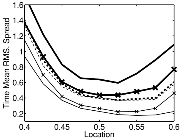
Fig. 4. rms error and spread from perfect model cases in Figs. 1–3, displayed only over the region where observations are available. Thick lines are rms and thin lines are spread. Solid lines are no inflation case (P-No), solid with ‘x’ are constant inflation (P-Con) and dashed are spatially varying adaptive inflation (P-ST).
