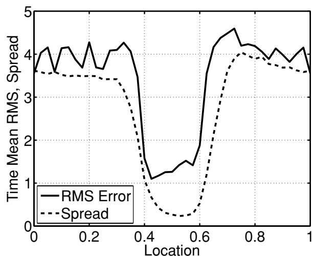
Fig. 7. As in Fig. 6 for case with an imperfect model and constant 1.09 inflation (case I-Con).
