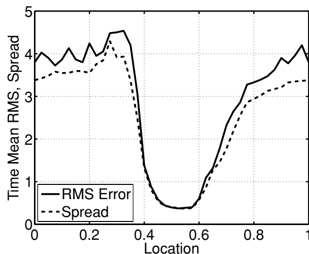
Fig. 3. As in Fig. 1 for case with a perfect model and spatially and temporally varying adaptive inflation (case P-ST).
