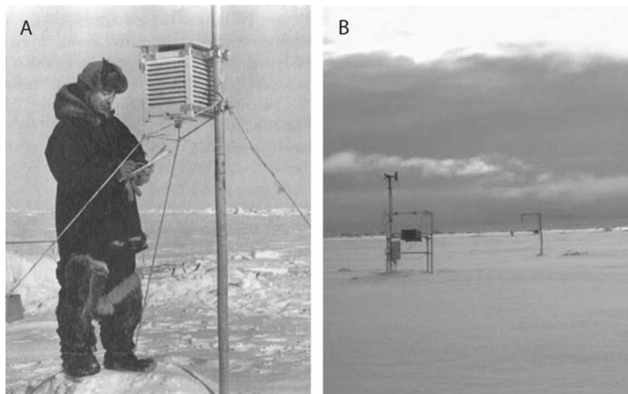
Fig. 1. Meteorological shelter for 2-m surface air temperatures from Russian North Pole (NP) station in 1937 and an autonomous station in 2003 from the North Pole Environmental Observatory (NPEO).
