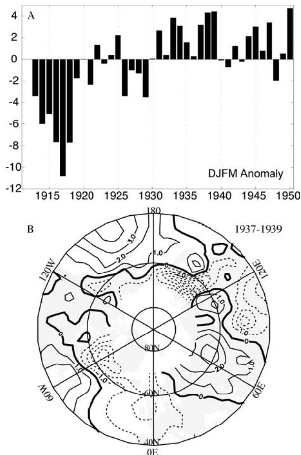
Fig. 7. (a) Winter (DJFM) SAT anomalies at Spitzbergen relative to a baseline period of 1912–2002. (b) Winter SLP anomalies for 1937–1939; Europe is in the lower margin of the figure with southerly geostrophic flow over northern Europe.
