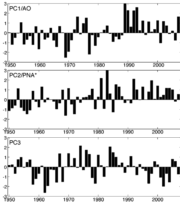
Fig. 5. Principal component time-series corresponding to Fig. 4 (right-hand side). Note the well-known positive AO (PC1) event in the early 1990s, the general shift in sign of the PNA* pattern (PC2) in the mid-1970s and the mostly negative values of PC3 from 1997–2004.
