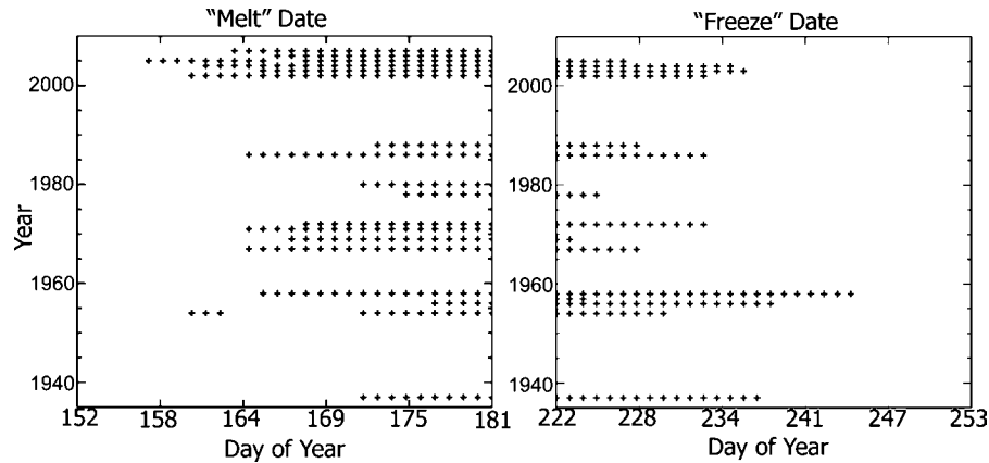
Fig. 2. Dates when NPEO SAT are above -2.0^{\circ}\text{C} for recent years (2002–2007), in contrast to those date from the Russian NP Stations (1937–1988). The mean transition date for this pseudo melt date is 7 d earlier for the recent NPEO observations relative to the NP Stations.
