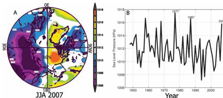
Fig. 10. (a) Summer (June–August) SLP field for 2007. Note the centre of high SLP over the Beaufort Sea. (b) Time history of summer SLP averaged over June–August for the area of 72.5–90°N and 90–180°W.
