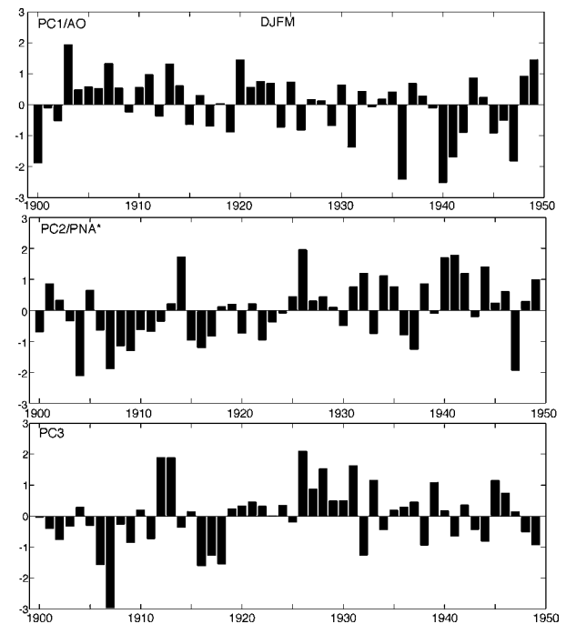
Fig. 6. Principal component time-series corresponding to Fig. 4 (left-hand side). Note the mostly positive AO from 1903–1925 and the general upward trend of the PNA*. PC3 has relatively large amplitudes from 1926–1933.
