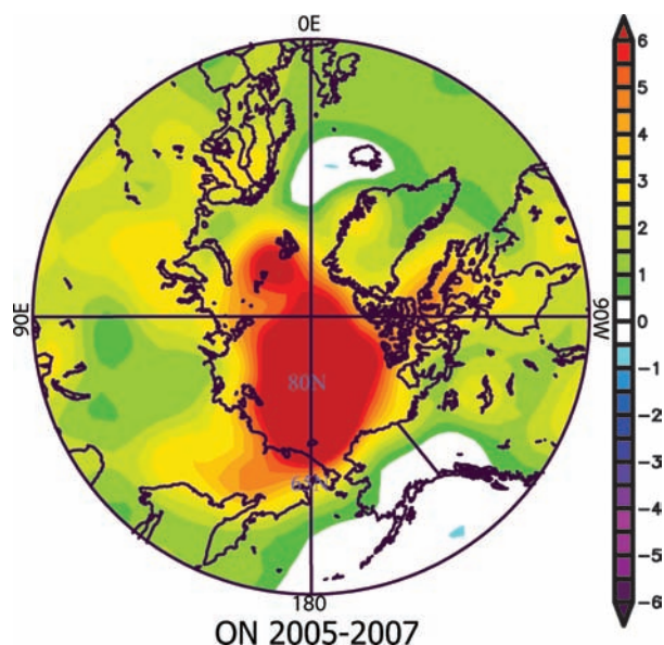
Fig. 11. Autumn (ON) SAT anomalies averaged for 2005–2007. Note the change in scale from previous figures with central Arctic values of greater than +6 °C.
