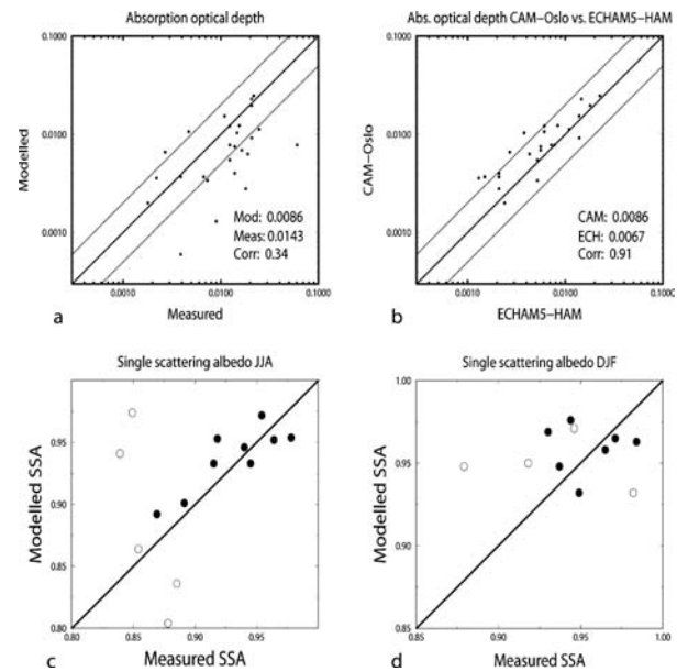
Fig. 20. Upper panel: Calculated versus observed aerosol absorption optical depth at 550 nm for (a) a selection of AERONET sites, and (b) compared with values from the model ECHAM5-HAM. Both measured and ECHAM5-HAM values are taken from Stier et al. (2005). Lower panel: Calculated versus observed values for the vertically integrated single scattering albedo at 550nm. The open circles are sites believed to be strongly influenced by emissions from biomass burning. The single scattering albedo is estimated as [1 - \text{ABS}/\text{AOD}] , where ABS is the absorption optical depth. The AOD are taken from the same dataset as presented in Figure 12.
