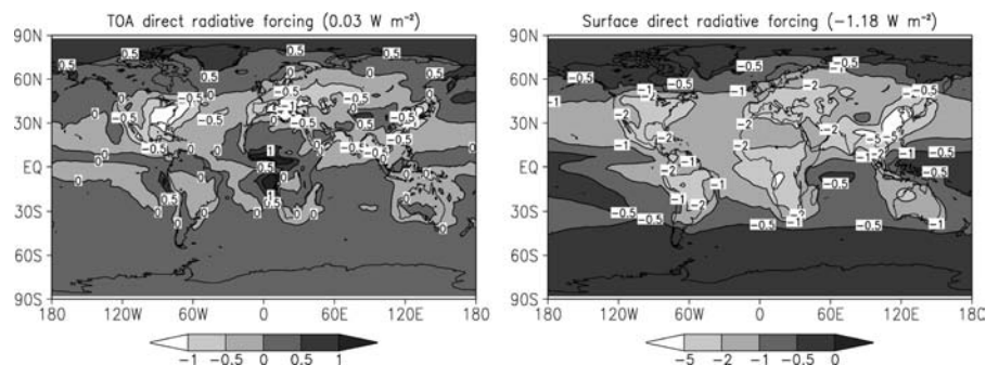
Fig. 14. Direct radiative forcing ( \text{W m}^{-2} ) due to anthropogenic aerosols at the top of the atmosphere (left) and at the surface (right).
