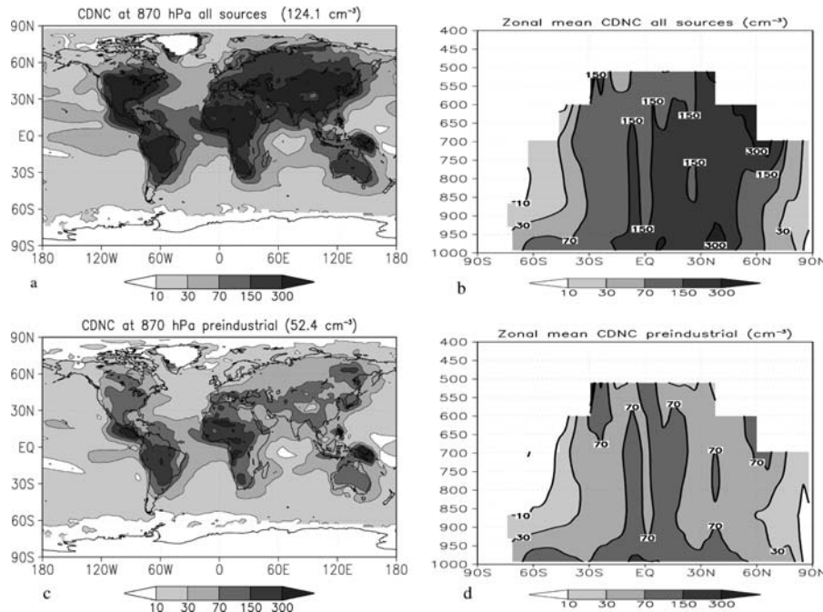
Fig. 15. Yearly averaged concentrations of cloud droplet number concentrations, CDNC ( \text{cm}^{-3} ) at model level \eta = 0.87 (a) and (c) to the left) and zonally averaged (b) and (d) to the right) for present day (upper panels) and pre-industrial (lower panels) emissions.
