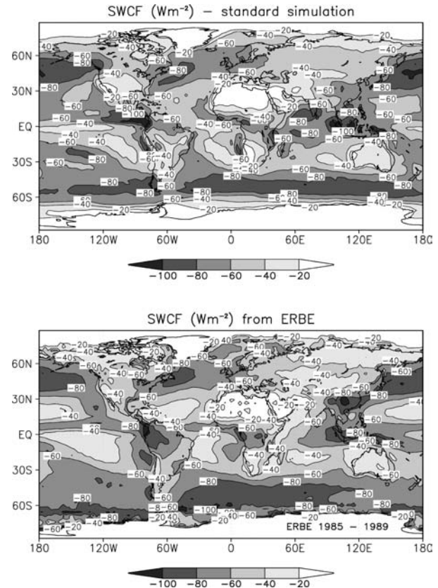
Fig. 18. Short-wave cloud forcing (SWCF, unit \text{W m}^{-2} ) in the control simulation (upper panel) and from the Earth Radiation Budget Experiment (ERBE, 1985–1989) (lower panel).
