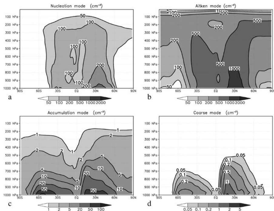
Fig. 9. Zonally averaged number concentrations ( \text{cm}^{-3} ) obtained using the definitions of aerosol modes given in Figure 1(a) the nucleation mode, (b) the aitken mode, (c) the accumulation mode and (d) the coarse mode.
