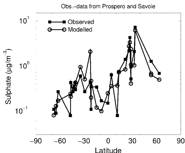
Fig. 5. Comparison of calculated and measured ground-level mass concentrations: Sulphate in remote oceanic areas (measurements obtained from Prospero and Savoie, pers. comm.).
