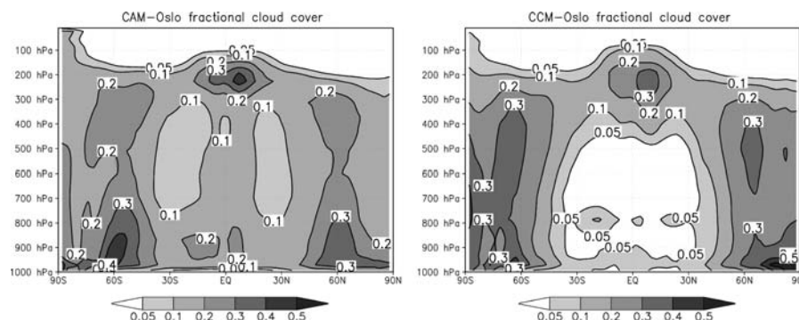
Fig. 2. Calculated zonally averaged fractional cloud cover in CAM-Oslo (left) and in CCM-Oslo (Kiehl et al., 1998; Kirkevåg et al., 2005) (right).
