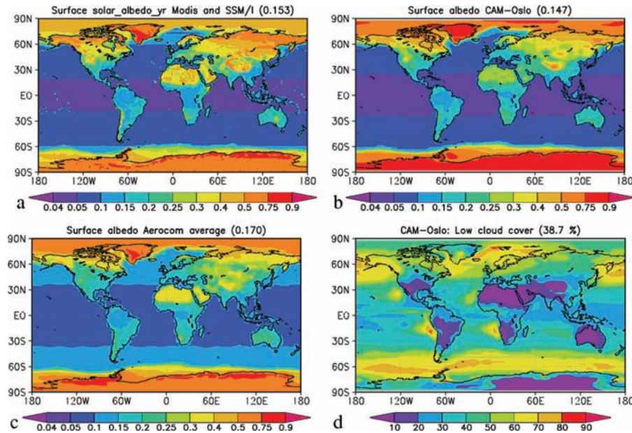
Fig. 21. (a) Surface albedo from Modis over land and calculated according to solar angle over sea; (b) Calculated surface albedo from CAM-Oslo; (c) Calculated surface albedo averaged for the AeroCom models and (d) Low-level cloud cover in CAM-Oslo. Data for a) and c) are obtained from S. Kinne (pers. comm.). The shown albedo data are for broadband solar radiation ( 0.2\text{--}5.0\ \mu\text{m} ).
