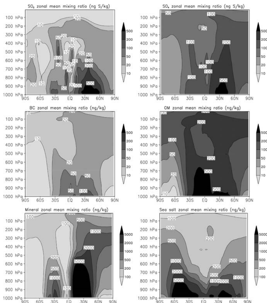
Fig. 4. Zonally averaged mass mixing ratios of \text{SO}_2 and aerosol components in the control simulation. Units: \text{ng (S) kg}^{-1} for \text{SO}_2 and \text{SO}_4 and \text{ng kg}^{-1} for the others.
