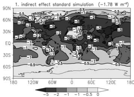
Fig. 17. Calculated first indirect radiative forcing ( \text{Wm}^{-2} ) for the control simulation.
