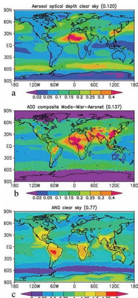
Fig. 11. Modelled and satellite retrieved aerosol optical depths (AOD) at 550nm. (a) Calculated clear-sky AOD, (b) Composite MODIS-MISR-AERONET AOD and (c) Clear-sky Ångström exponent (ANG).
