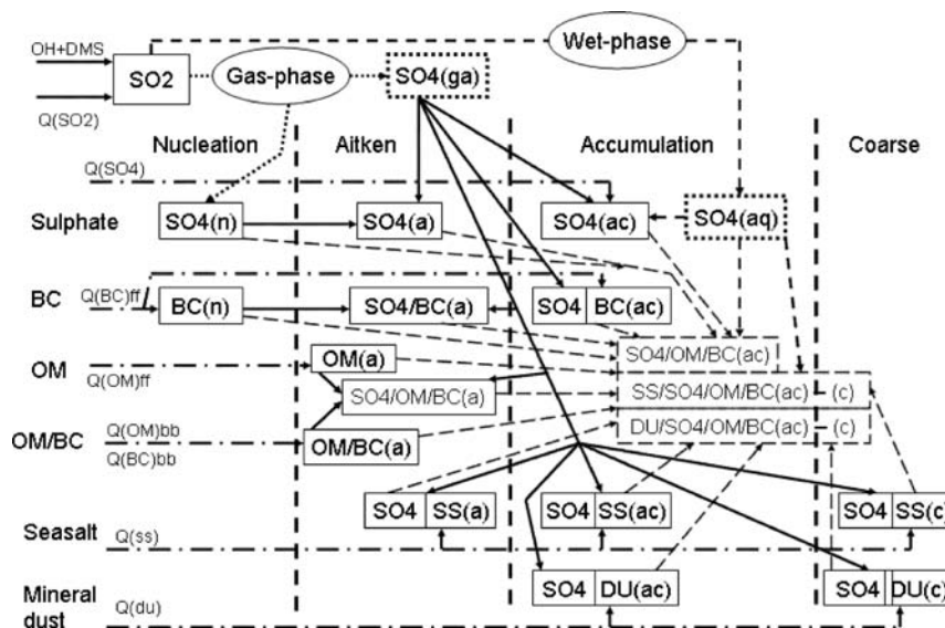
Fig. 1. Schematic for aerosol particle processing in CAM-Oslo. Primary particles are emitted (dashed-dotted arrows) as accumulation-mode sulphate ( \text{SO}_4(\text{ac}) ), nucleation and accumulation mode black carbon ( \text{BC}(\text{n}) , \text{BC}(\text{ac}) ), aiten mode organic matter, ( \text{OM}(\text{a}) ), internally mixed aiten mode OM and BC ( \text{OM/BC}(\text{a}) ), aiten, accumulation, and coarse mode sea-salt ( \text{SS}(\text{a}) , \text{SS}(\text{ac}) , \text{SS}(\text{c}) ), accumulation and coarse mode mineral dust ( \text{DU}(\text{ac}) , \text{DU}(\text{c}) ). Model calculated gas-phase components are DMS and \text{SO}_2 . Gaseous sulphate ( \text{SO}_4(\text{ga}) ) produced in clear air is immediately transformed to nucleation-mode sulphate ( \text{SO}_4(\text{n}) , dotted arrow) in cases when there is insufficient pre-existing particle surface area available for condensation (continuous arrows). Sulphate produced by oxidation in cloud droplets ( \text{SO}_4(\text{aq}) , short-dashed arrow) is partly added to \text{SO}_4(\text{ac}) but mainly to a broad internal mixture of accumulation and coarse mode particles (compounds in dashed rectangles of which there are three types). Long-dashed arrows represent coagulation processes also contributing to the latter particle types.
