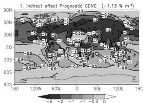
Fig. 19. As Figure 17, except that a prognostic equation for cloud droplet number concentrations is used. Unit: \text{W m}^{-2} .
