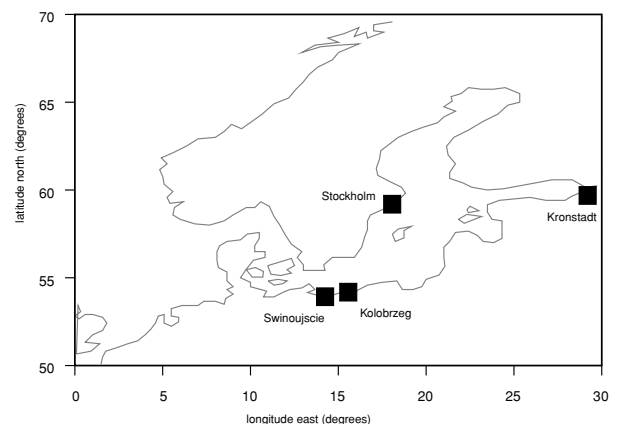
Fig. 1. Sketch of the Baltic Sea, showing the location of the four sea level gauges used in this study.
