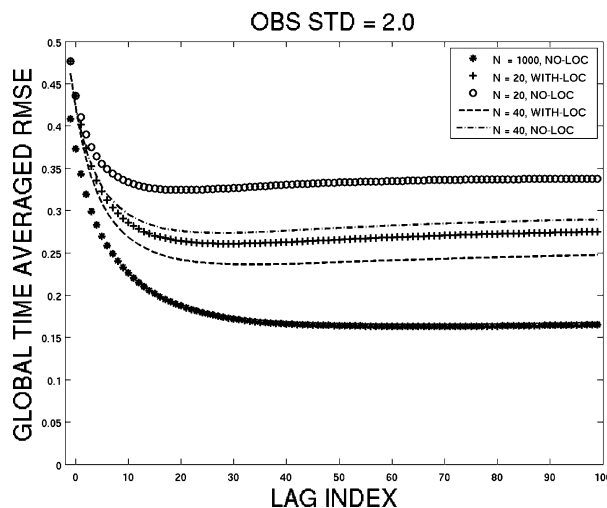
Fig. 3. Results for the Lorenz 1996 OSSEs for large observational error standard deviation with an identity observing network. The y-axis depicts the global time mean root mean squared error between the true system state and the ensemble mean estimate versus LAG INDEX on the x-axis. Results are shown for ensemble sizes N = 1000 , 40 and 20 where no localization in the smoother update step is used, as well as for N = 40 and 20 where localization is used in the smoothing update step.
