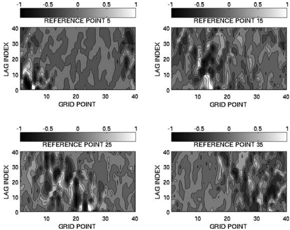
Fig. 2. Results for the Lorenz 1996 OSSEs for small observational error standard deviation with an identity observing network. The ensemble size is N = 1000 . The upper-left-hand panel depicts the one-point prior correlations with increasing LAG INDEX vertically, and GRID POINT horizontally where the reference GRID POINT is 5. The correlation coefficients are computed for the prior ensemble at GRID POINT 5 at time t_i and another grid point at t_i - (\text{LAGINDEX}) . For larger values of LAG INDEX, the absolute values of the correlation coefficients are highest, upstream of the reference point, consistent with the dynamics of small perturbations in the Lorenz 1996 model. The remaining panels are analogous, except the reference point has been changed.
