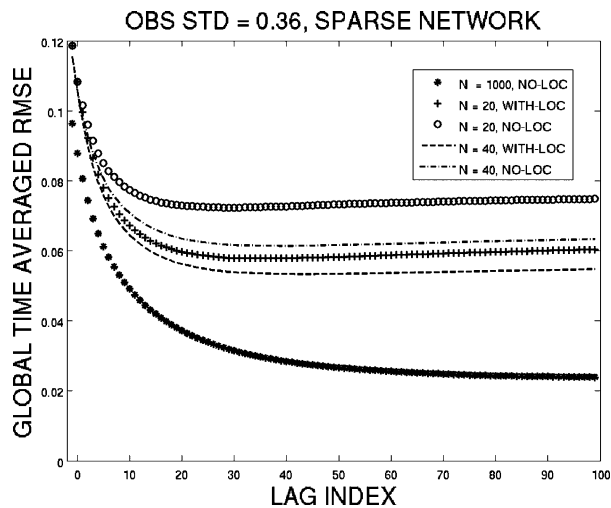
Fig. 4. Results for the Lorenz 1996 OSSEs for small observational error standard deviation with a 'SPARSE' observing network which consists of observations of every second state variable. The y-axis depicts the global time mean root mean squared error between the true system state and the ensemble mean estimate versus LAG INDEX on the x-axis. Results are shown for ensemble sizes N = 1000 , 40 and 20 where no localization in the smoother update step is used, as well as for N = 40 , 20 where localization is used in the smoothing update step.
