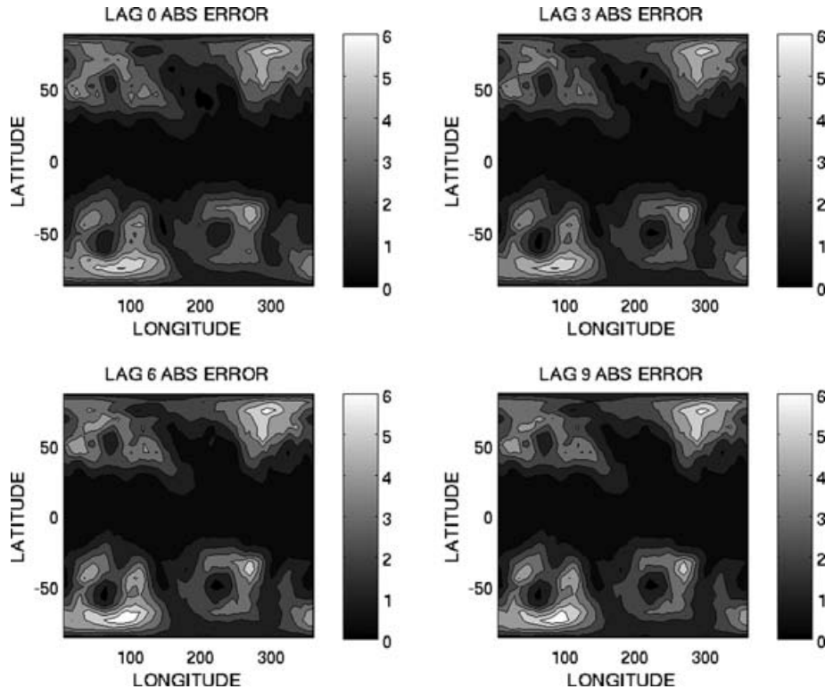
Fig. 10. Results for the Atmospheric General Circulation Model with N = 50 , where localization has been used in the smoother update steps. The upper-left-hand panel is a contour plot which depicts the time mean absolute errors at the PS grid points for the posterior errors ( LAG = 0 ). The upper-right-, lower-left- and lower-right-hand panels depict the analogous results for LAG = 3, 6 and 9 , respectively. One LAG unit is equal to 12 h.
