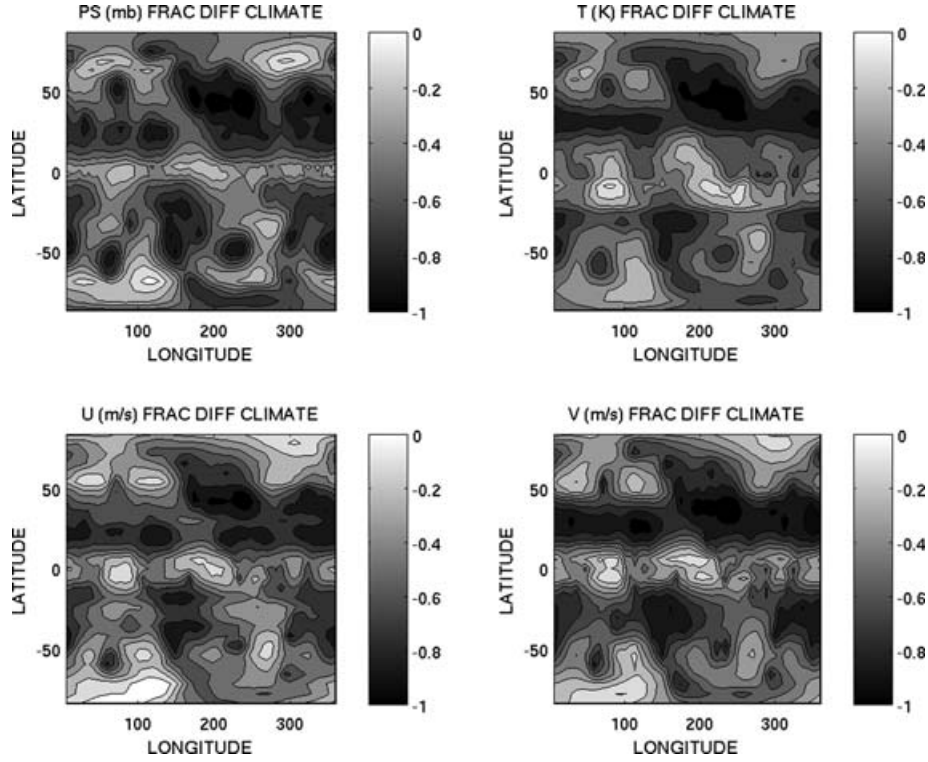
Fig. 7. The upper-left-hand panel depicts results for the surface pressure PS . At each model grid point, the fractional difference between the time mean absolute posterior error in the OSSE and a free climatological run has been computed. The panels depict contour plots of the fractional differences. The remaining panels depict results for the temperature T , zonal and meridional winds U and V .
