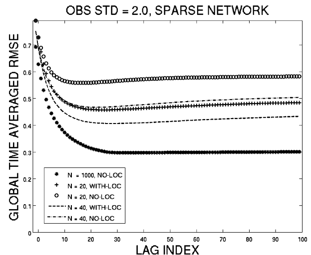
Fig. 5. Results for the Lorenz 1996 OSSEs for large observational error standard deviation with a 'SPARSE' observing network which consists of observations of every second state variable. The y-axis depicts the global time mean root mean squared error between the true system state and the ensemble mean estimate versus LAG INDEX on the x-axis. Results are shown for ensemble sizes N = 1000 , 40 and 20 where no localization in the smoother update step is used, as well as for N = 40 and 20 where localization is used in the smoothing update step.
