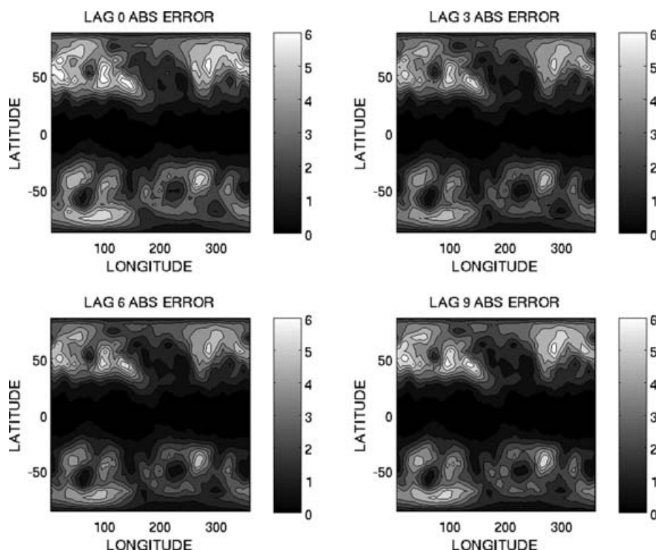
Fig. 9. Results for the Atmospheric General Circulation Model with N = 20 , where localization has been used in the smoother update steps. The upper-left-hand panel is a contour plot which depicts the time mean absolute errors at the PS grid points for the posterior errors ( LAG = 0 ). The upper-right-, lower-left- and lower-right-hand panels depict the analogous results for LAG = 3, 6 and 9 , respectively. One LAG unit is equal to 12 h.
