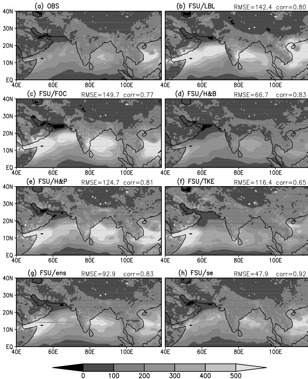
Fig. 4. Geographical distribution of Day 1 forecast of latent heat flux ( \text{Wm}^{-2} ) for 17 Aug 2002 over the monsoon domain ( 40^{\circ}\text{E} – 120^{\circ}\text{E} , \text{Eq} – 40^{\circ}\text{N} ).
