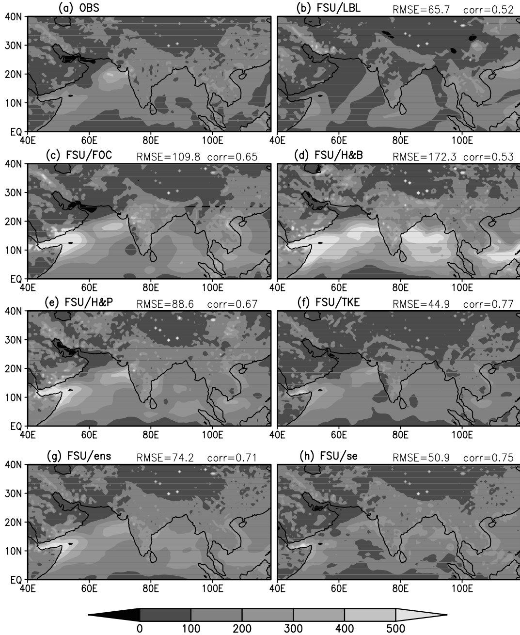
Fig. 5. Geographical distribution of Day 1 forecast of latent heat flux ( \text{Wm}^{-2} ) for 26 Aug 2002 over the monsoon domain (40°E–120°E, Eq–40°N).
